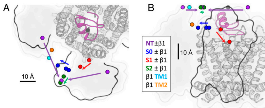
Fig. 6. Change in the donor position due to the presence of the \beta 1 -subunit. (A and B) Top and side views, respectively, of the changes in the donor positions as a consequence of coexpression with the \beta 1 -subunit. The 95% confidence isosurfaces are not displayed for clarity. Colored arrows indicate the direction of the change in position.
