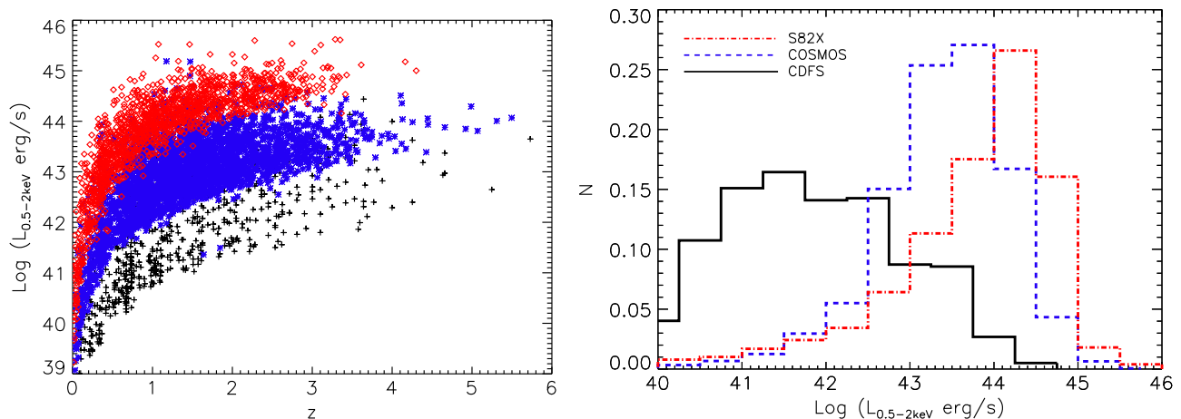
Figure 14. Left: K -corrected (rest-frame) soft-band (0.5–2 keV) luminosities as a function of redshift for the Stripe 82X (red diamonds), COSMOS-Legacy (blue asterisks; Civano et al. 2015; Marchesi et al. 2015), and CDFS (black crosses) sources. At every redshift, an increase in survey area preferentially identifies higher-luminosity sources. Right: normalized distribution of k -corrected soft-band luminosities for Stripe 82X compared with COSMOS and CDFS: the wide-area coverage of Stripe 82X which probes a large effective volume of the universe, enables the rare, highest luminosity quasars to be uncovered, complementing the parameter space explored by small- to moderate-area surveys. In both plots, only the sources identified with redshifts are plotted, representing 30% of the Stripe 82X sample (which currently has only spectroscopic redshifts) and 91% and 96% of the CDFS and COSMOS-Legacy sample, respectively, where both spectroscopic and photometric redshifts are available.
