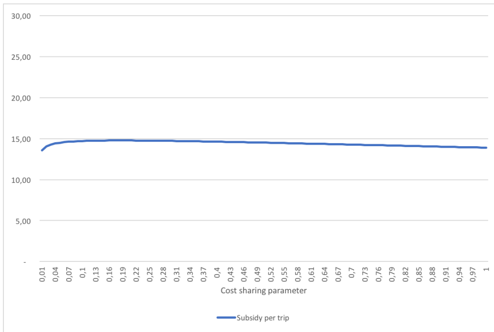
Figure 2: Subsidy per trip: model 1
