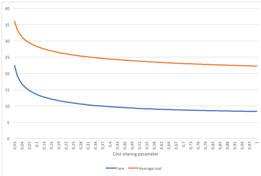
Figure 1: Average cost and optimal fare: model 1
