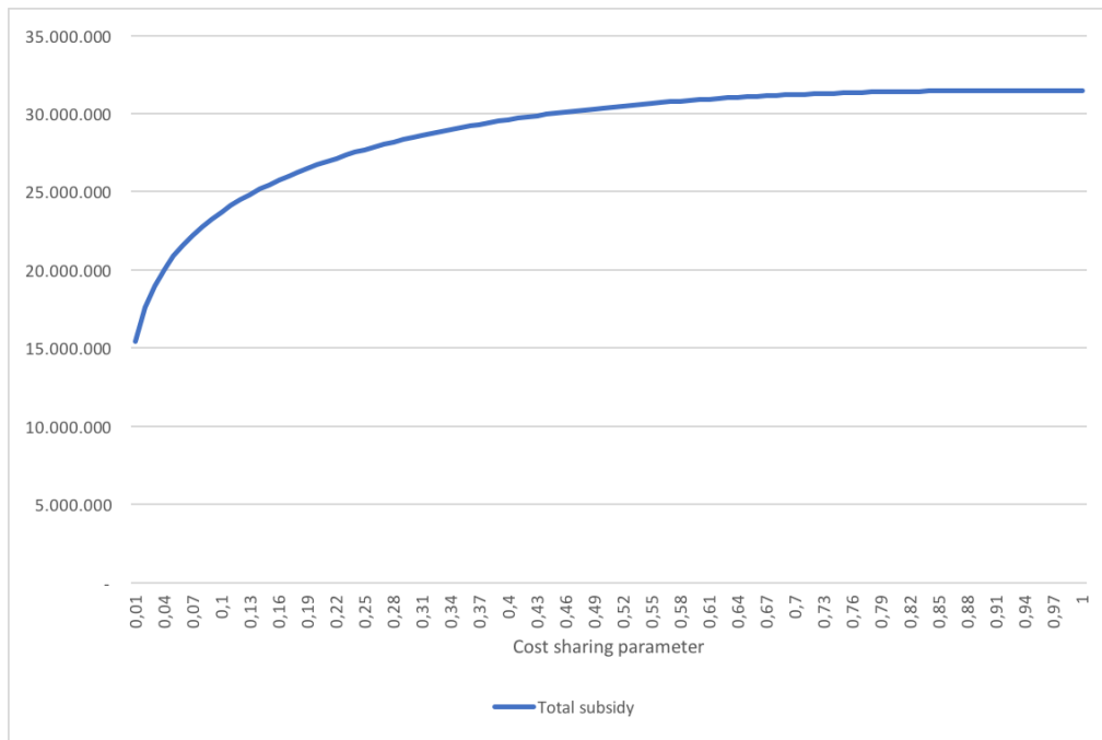
Figure 3: Total Subsidy: model 1
