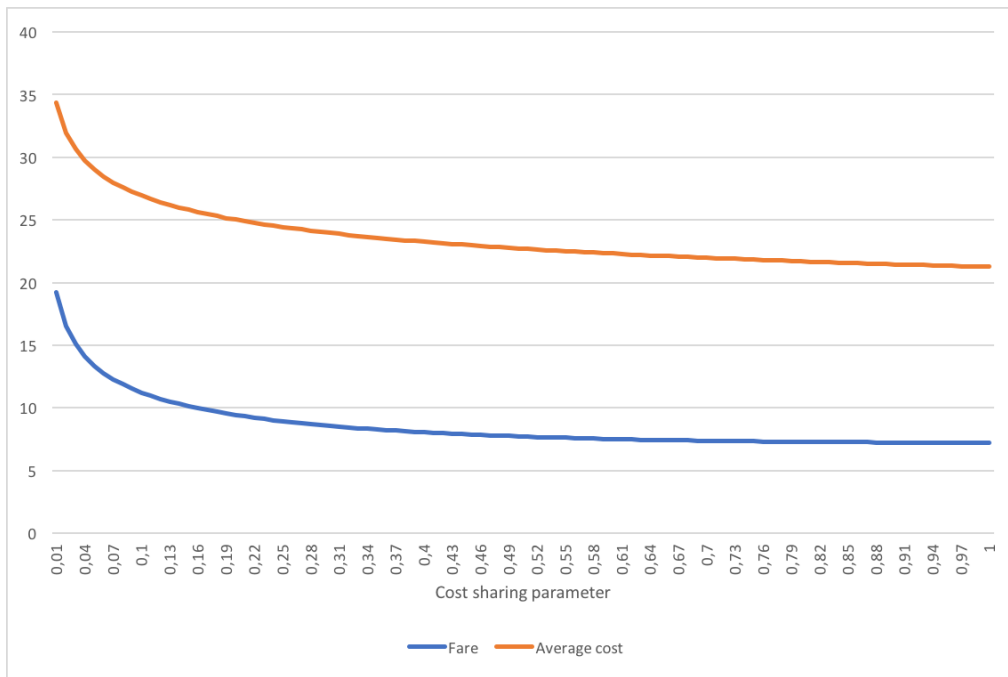
Figure 4: Average cost and optimal fare: model 2
