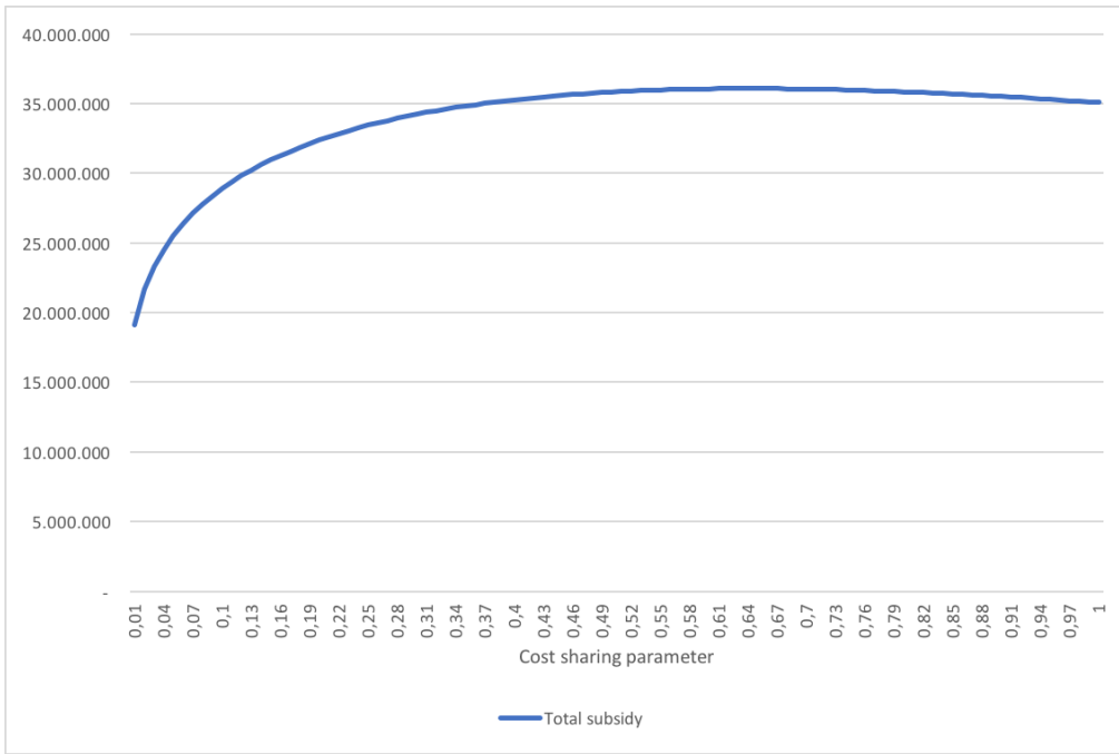
Figure 6: Total Subsidy: model 2
