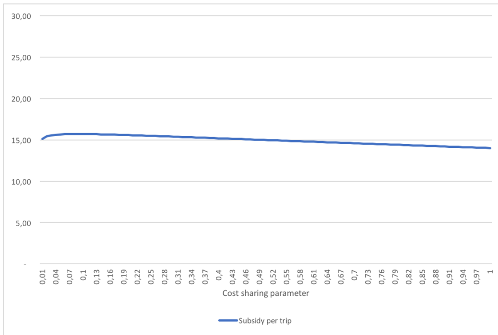
Figure 5: Subsidy per trip: model 2
