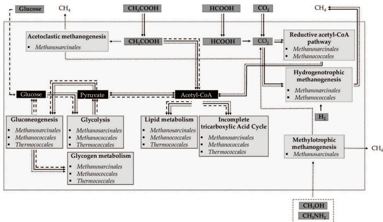
Figure 2. The simplified scheme of Euryarchaeal metabolism. Thermococcales are used as an example to represent heterotrophic archaea, Methanococcales as an example of class I methanogens and Methanosarcinales of class II methanogens. Light gray squares represent main metabolic processes mentioned in the text. The genera carrying each process are enclosed in a square. The relevant metabolites that can enter the cell are represented in dark gray squares. Metabolites that serve as intermediaries and connecting different processes are represented by black squares. \text{CH}_4 , one of the major metabolic final products from methanogenic archaea is shown. The arrows represent connections between metabolites and metabolic processes. The dashed arrows represent the pathways present in Thermococcales ; the black arrows represent the pathways present in Methanococcales , and the dotted arrows represent the pathways present in Methanosarcinales .
