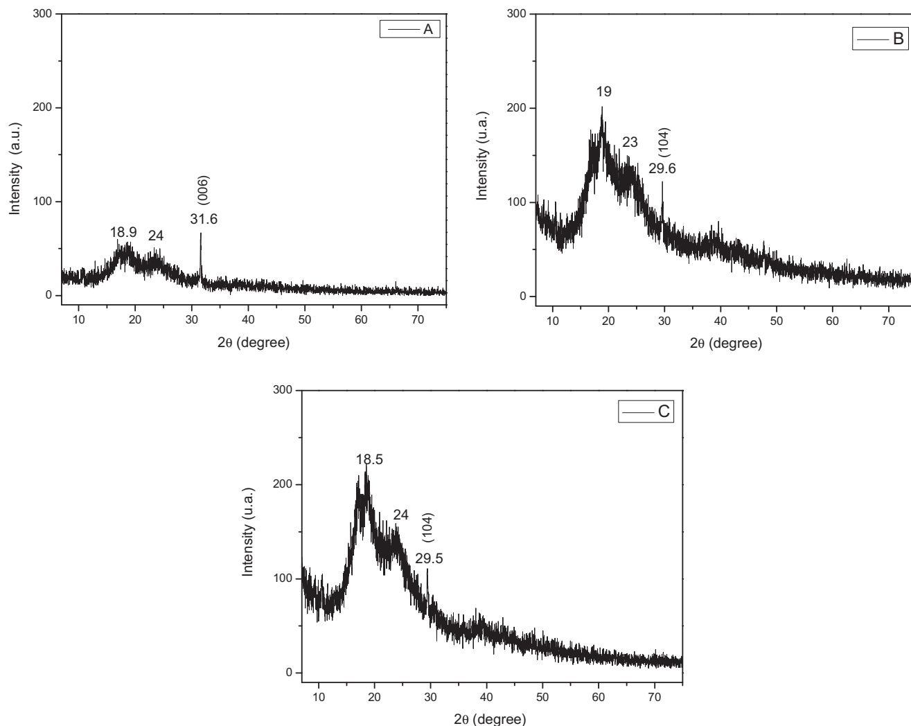
Fig. 9. XRD patterns of \text{CaCO}_3 particles grown using GD after 24 h in the presence of: A) PA as additive (control), B) sponge matrix (control), and C) sponge plus PA.
