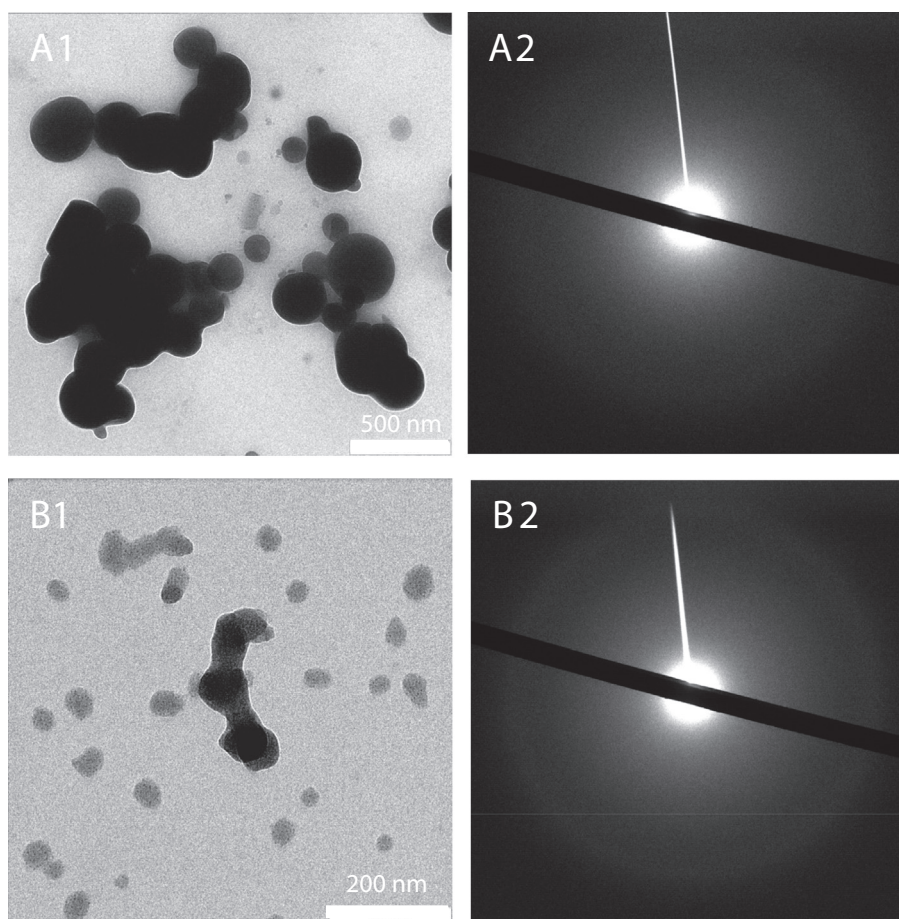
Fig. 7. TEM micrographs and electron diffraction patterns of \text{CaCO}_3 particles grown using the GD method with PA after 15 min mineralization time on A) gastrogel and B) sponge matrices.
