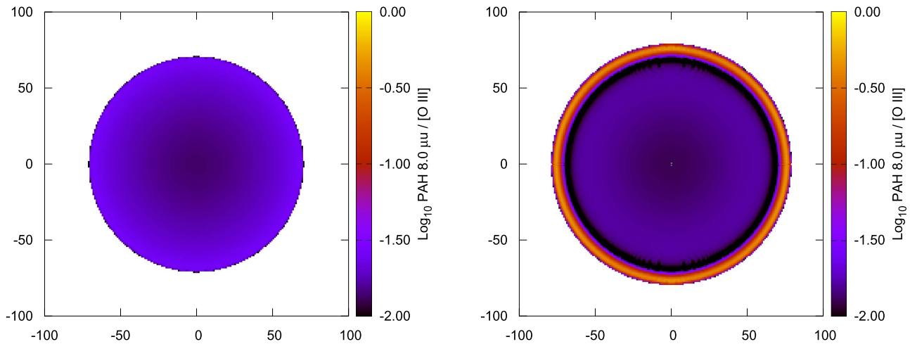
Figure 1. Modeled 8\ \mu\text{m}/[\text{O III}] ratio map of an LMC H II region ionized by an O6 V star, for \tau = 0.5 (left) and \tau = 20 (right). The assumed parameters are the same as in Figure 2 of Pellegrini et al. (2012), with x - and y -axes showing spatial projection in arcsec at the LMC distance. PAHs survive and dominate emission near the Strömgen edge in the optically thick object, in contrast to the optically thin object.
