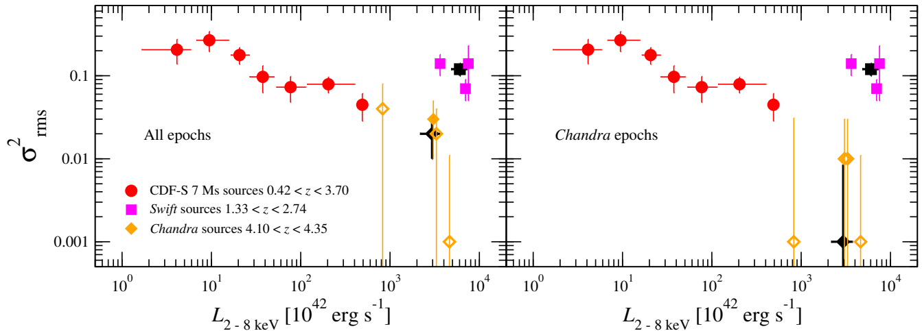
FIG. 2.— Excess variance versus luminosity in the rest-frame 2–8 keV band. Circles represent average luminosities and \sigma_{\text{rms}}^2 values of X-ray-selected AGNs, grouped in seven luminosity bins, from the 7 Ms exposure of the CDF-S survey (adapted from P17). Squares and diamonds represent the Swift and Chandra sources, respectively; open diamonds mark non-variable Chandra sources. Sources with negative \sigma_{\text{rms}}^2 values have been pegged at \sigma_{\text{rms}}^2 = 0.001 . Error bars on \sigma_{\text{rms}}^2 represent ‘formal’ errors due only to flux measurement errors and not those due to red-noise intrinsic scatter. The black diamond and square represent the average \sigma_{\text{rms}}^2 and L_{2-8 \text{ keV}} values of our Chandra and Swift sources, respectively. The left (right) panel represents all (only the Chandra ) epochs.
