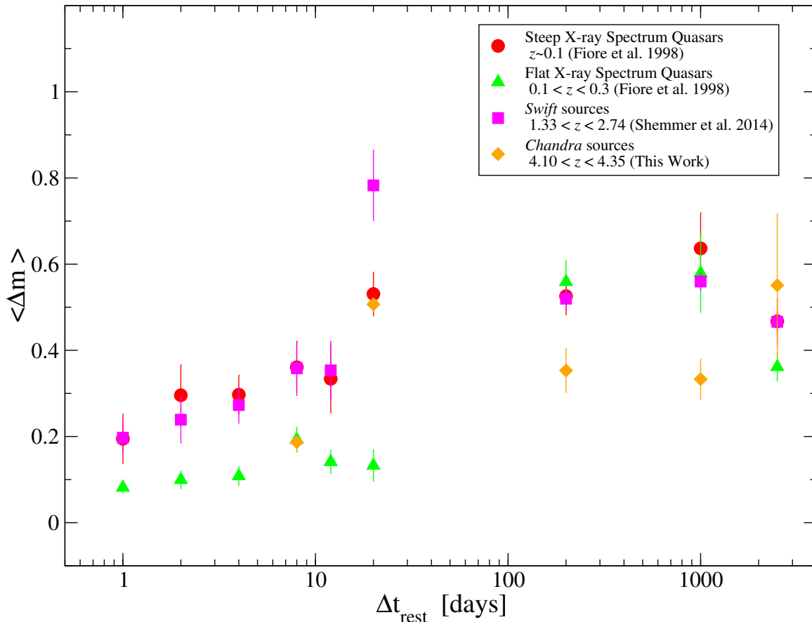
FIG. 4.— Ensemble SF of the Chandra sources (diamonds) compared to the ensemble SF of the Swift sources from Paper I (squares) as well as the ensemble SFs of the steep- and flat-X-ray-spectrum quasars at low redshift, marked by circles and triangles, respectively, adapted from Fiore et al. (1998). Average magnitude difference in each time bin is plotted as a function of rest-frame time interval. Except for the longest timescale, the ensemble SF of sources at z \simeq 4.2 is significantly lower than that of similarly luminous RQQs at intermediate redshifts.
