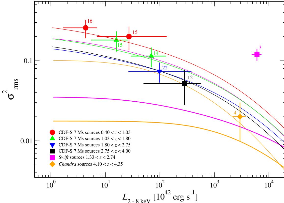
FIG. 3.— Similar to the left panel of Fig. 2, except that the CDF-S sources are binned into four redshift intervals. Circles, upward triangles, downward triangle, and filled square represent average luminosities and \sigma_{rms}^2 values of X-ray-selected AGNs from the 7 Ms exposure of the CDF-S survey at 0.40 < z < 1.03 , 1.03 < z < 1.80 , 1.80 < z < 2.75 , and 2.75 < z < 4.00 , respectively (adapted from P17). The magenta square and orange diamond represent the average luminosities and \sigma_{rms}^2 values of our Swift and Chandra sources, respectively (with six epochs, per source, considered for the latter). The number of sources is indicated next to each bin. Red, green, blue, and black thin solid lines represent the most acceptable \sigma_{rms}^2 vs. L_{2-8\text{ keV}} models, having L/L_{Edd} = 0.04, 0.06, 0.09 , and 0.08 , corresponding to the bins with matching color, in order of increasing redshift. The magenta and orange thin (thick) solid lines represent similar models corresponding to the Swift and Chandra bins, respectively, but having L/L_{Edd} = 0.06 ( L/L_{Edd} = 0.50 ). The models with higher Eddington ratios predict smaller variability amplitudes at a given luminosity.
