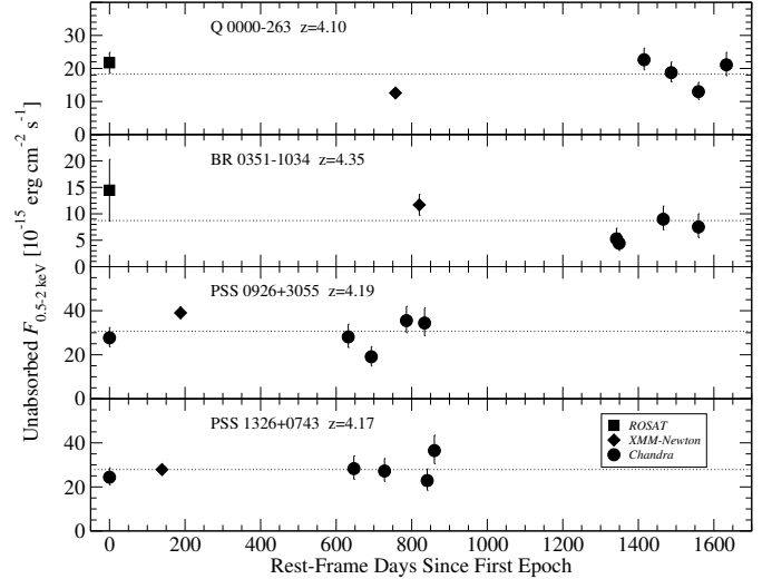
FIG. 1.— X-ray light curves of the Chandra sources. Galactic absorption-corrected flux in the soft band (i.e., the observed-frame 0.5–2 keV band) is plotted as a function of rest-frame time (in days) relative to the first X-ray epoch for each source. Squares, diamonds, and circles mark ROSAT, XMM-Newton, and Chandra observations, respectively. The dotted line in each panel indicates the mean flux.
