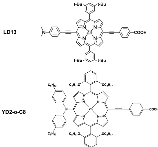
Fig. 1 Molecular structures of LD13 and YD2-o-C8 dyes porphyrins.
