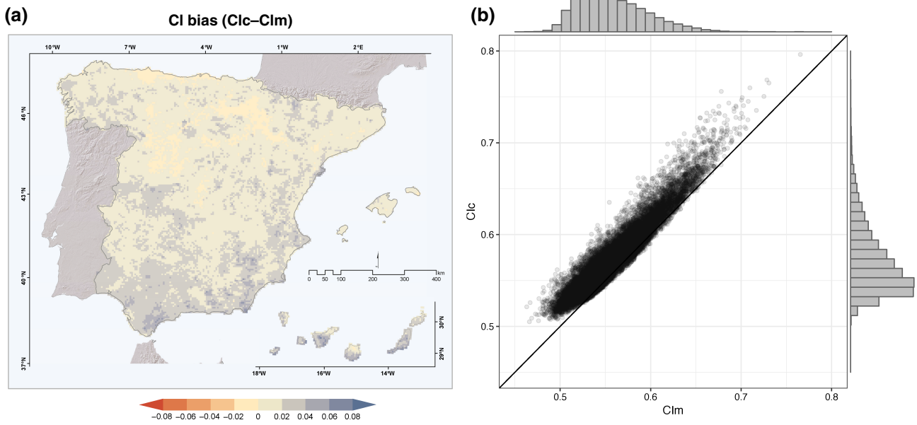
Figure 4. (a) CI bias (CIc-CIm) spatial distribution and (b) scatterplot of averaged annual CI values (CIm) versus the CI computed with complete series (CIc). Dots represent the grid points covering Spain, the black line shows the optimal fit where both variables give the same values, and histograms show the frequencies of values.
