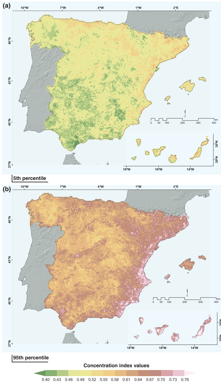
Figure 6. (a) Fifth and (b) 95th percentile of annual CI values.
