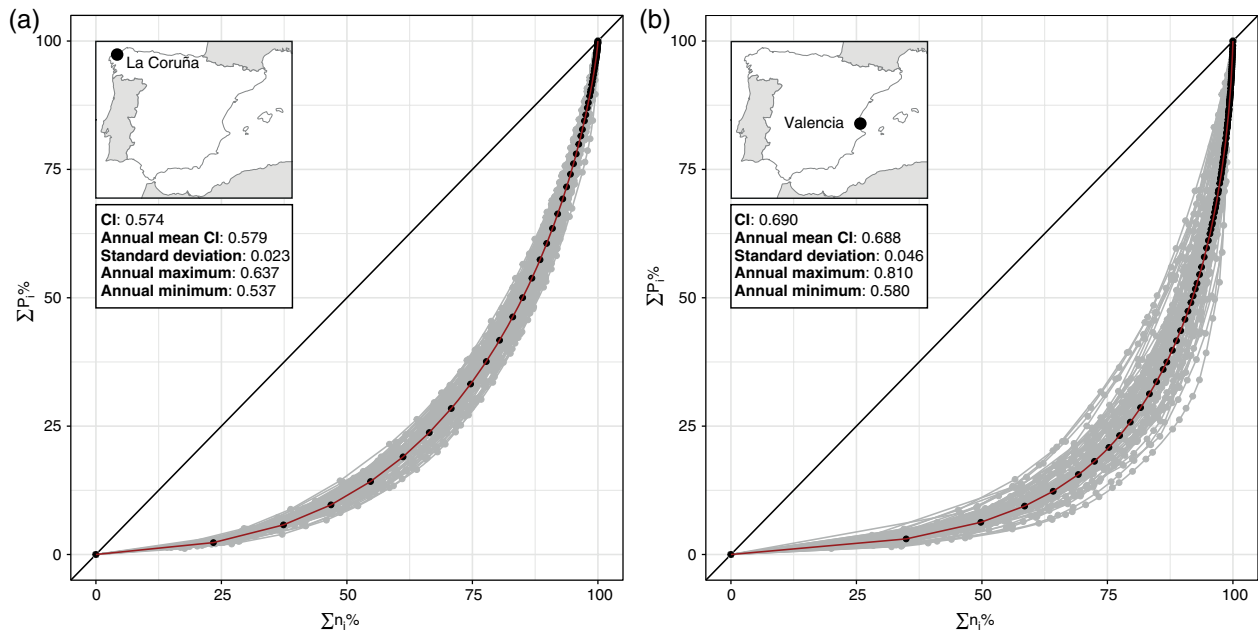
Figure 2. Cumulative percentage of rainy days ( \Sigma n_1\% ) versus the cumulative percentage of rainfall amounts ( \Sigma P_1\% ) in (a) La Coruña and (b) Valencia. Black dots with red lines are the exponential curves using complete series, and grey dots and lines are the annual exponential curves.
