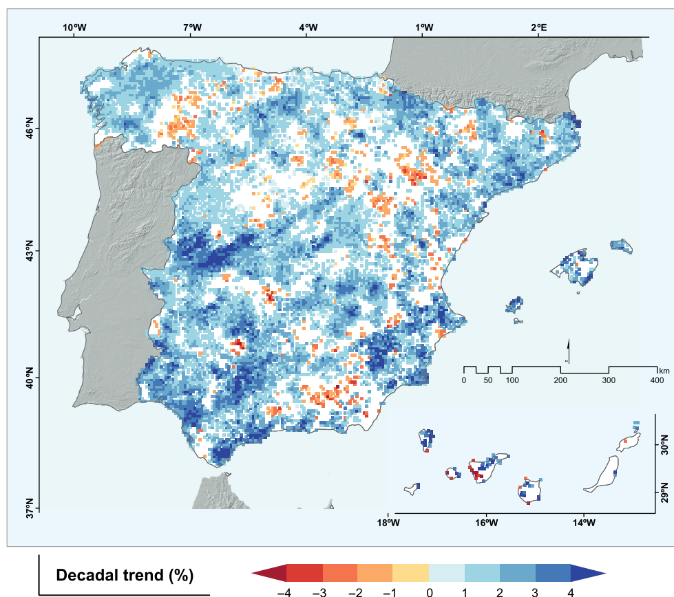
Figure 7. Percentage of change by decade of annual CI in Spain (1950–2012). Only significant trends ( p < 0.05 ) are represented in colour, while non-significant areas are left white.
