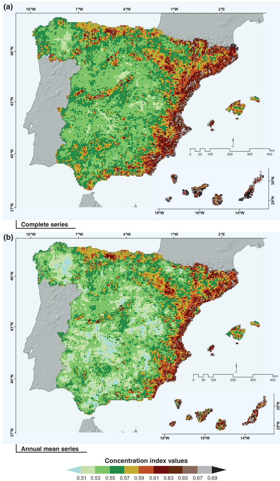
Figure 3. PCI in peninsular Spain (1950–2012), and the Balearic and Canary Islands (1971–2012) using (a) complete series (CIc) and (b) mean annual series (CI m ).
