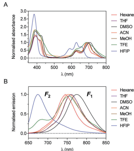
Fig. 2 Absorption (A) and emission spectra (B, \lambda_{\text{exc}} = 598 nm) of ATAZPo 2 in different solvents.
