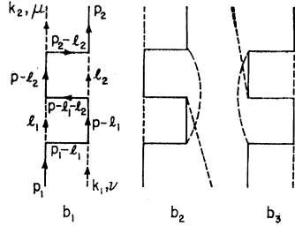
FIG. 4. Relevant diagrams for sixth-order Compton scattering.
