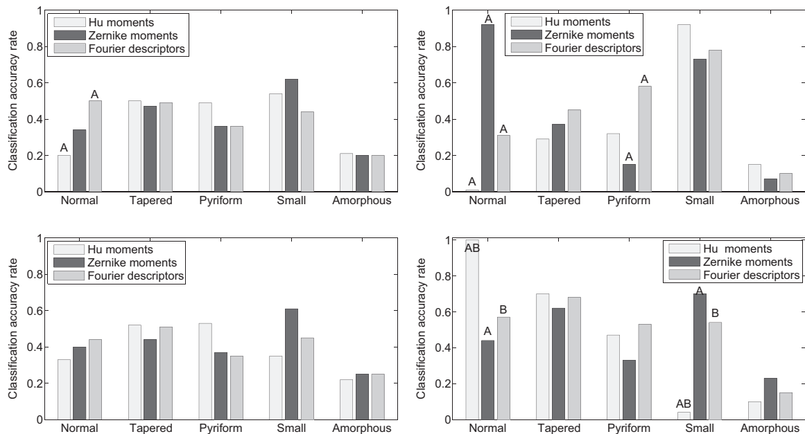
Fig. 6. Five-class base-line classification. We compare the results obtained using four different classification approaches: 1 – NN (top left), naive Bayes (top right), decision trees (bottom left) and SVM (bottom right). Statistical differences between descriptors in each class were considered significant at p < 0.05 and indicated as A and B. For instance, in fourth row, for class Normal, the A in Hu moments and Zernike moments means that there is a significant difference between those descriptors, while the B in Hu moments and Fourier descriptors means that there is a significant difference between those descriptors.
