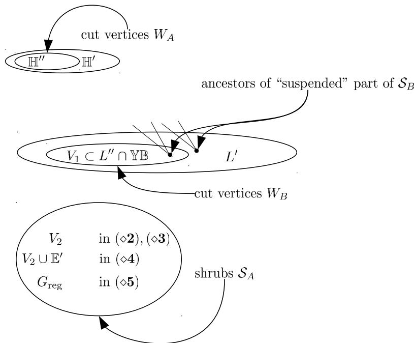
FIG. 2. An overview of embedding of a tree T \in \text{trees}(k) given with its fine partition (W_A, W_B, \mathcal{S}_A, \mathcal{S}_B) using configurations (\diamond 2) – (\diamond 5) . The hubs are embedded between \mathbb{H}'' and V_1 , and all the shrubs \mathcal{S}_A are embedded in sets specific to particular configurations so that the vertices neighboring the seeds W_A are embedded in V_1 . Parts of the shrubs \mathcal{S}_B are embedded directly (using various embedding techniques), while the rest are “suspended,” i.e., the ancestors of the unembedded remainders are embedded on vertices which have large degrees in \mathbb{H}' . The embedding of \mathcal{S}_B is then finalized in the last stage.
