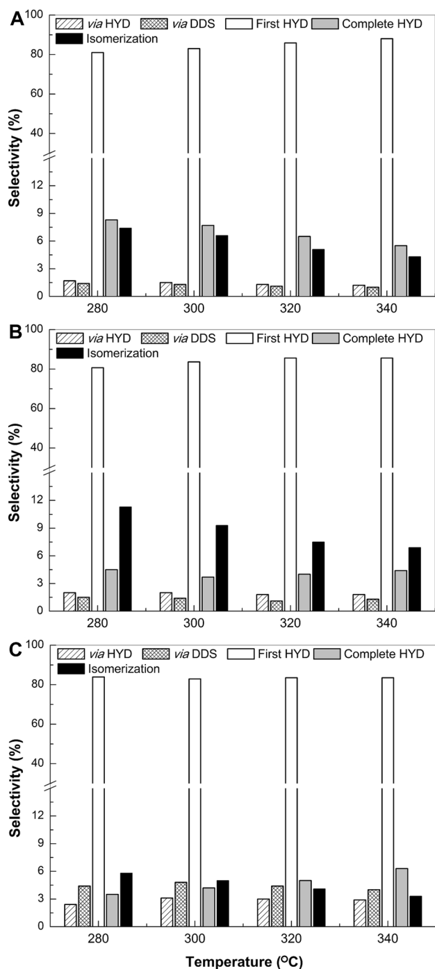
Fig. 8 Selectivity taken to 20–25% of 3-methyl-thiophene conversion of the ReS 2 samples annealed at 400 °C (a), 800 °C (b) and Mo/γ-Al 2 O 3 (c)
