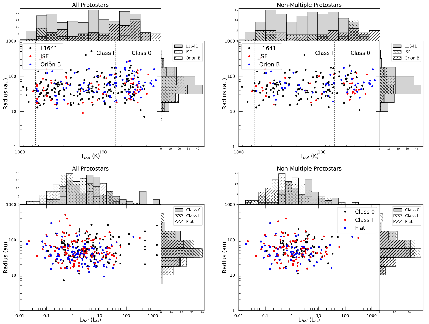
Figure 10. Comparison of protostellar disk radii to T_{bol} (top panels) and L_{bol} (bottom panels). The accompanying histograms in the top panels separate the sample by their region and in the bottom panels the sample is separated by class. The colorization and histograms associated with the top panels separates the sources by their regions (black: L1641, red: integral-shaped filament [ISF], blue: Orion B). In the bottom panels, the colors and associated histograms separate the sources by class; black corresponds to Class 0 protostars, red corresponds to Class I protostars, and blue corresponds to Flat spectrum protostars. The left panels show the full sample with a corresponding measurement of L_{bol} and T_{bol} , while the right panels show only non-multiple sample. There is no strong correlation between disk radii and T_{bol} or L_{bol} .
