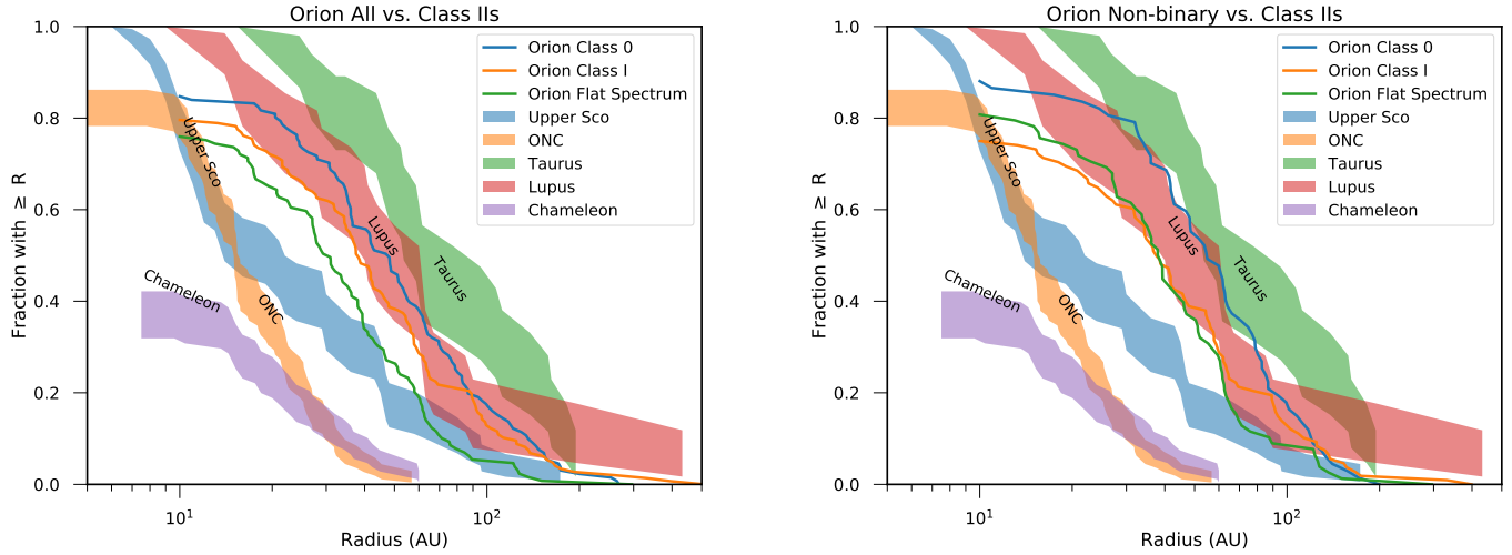
Figure 16. Cumulative distributions of disk radii within the Orion sample (lines) compared to Class II disk samples. The left panel shows the full sample, while the right panel only shows the non-multiple sample. The Orion protostellar disk radii are larger than those of Class II disks in most regions, comparable to Lupus, but smaller than Taurus. This, in addition to the radius comparison within Orion, suggests that there may not be a monotonic growth of disks from the protostellar to Class II disk phase.
