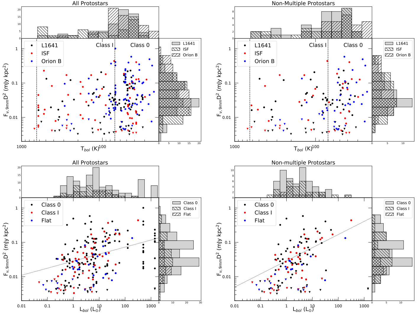
Figure 7. Same as Figure 6, but comparing the 9 mm flux densities. The lines in the lower panels are the fits to the 9 mm flux densities versus L_{bol} , for the full sample (left panel) we find F_{\nu} D^2 \propto L_{bol}^{0.2 \pm 0.03} and for the non-multiple sample (right) we find F_{\nu} D^2 \propto L_{bol}^{0.38 \pm 0.07} .
