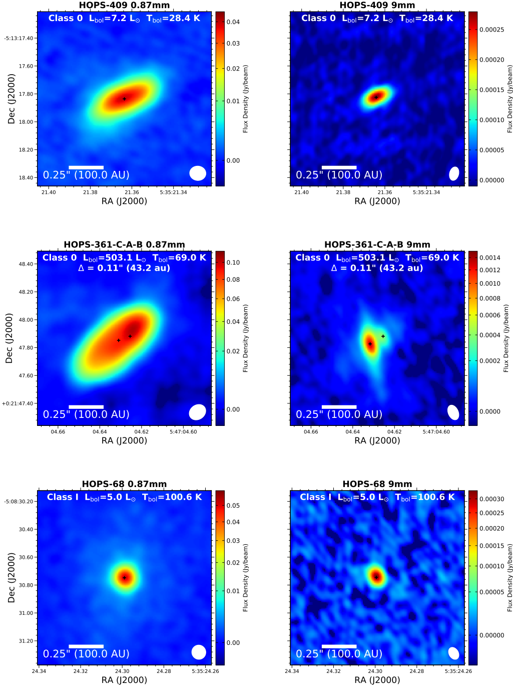
Figure 3. Example images from ALMA (left) at 0.87 mm and the VLA (right) at 9 mm toward selected sources. The top row shows HOPS-409, a Class 0 protostar with an apparent resolved disk at 0.87 mm and 9 mm. HOPS-361-C, a high-luminosity Class 0 source, is shown in the middle row and appears disk-like at 0.87 mm. However, HOPS-361-C is resolved into a close binary system by the VLA at 9 mm. The brighter source also exhibits an extended free-free jet at this wavelength. HOPS-68, a Class I source, is shown in the bottom row and appears compact and only marginally resolved at both 0.87 mm and 9 mm. The synthesized beams are drawn in the lower right; the typical ALMA synthesized beam is 0''.1 and the typical VLA beam is 0''.08 . Images for the remaining protostars are shown in Appendix C. A blank panel for the ALMA 0.87 mm or VLA 9 mm panel means that observations were not taken that particular protostar with ALMA or the VLA.
