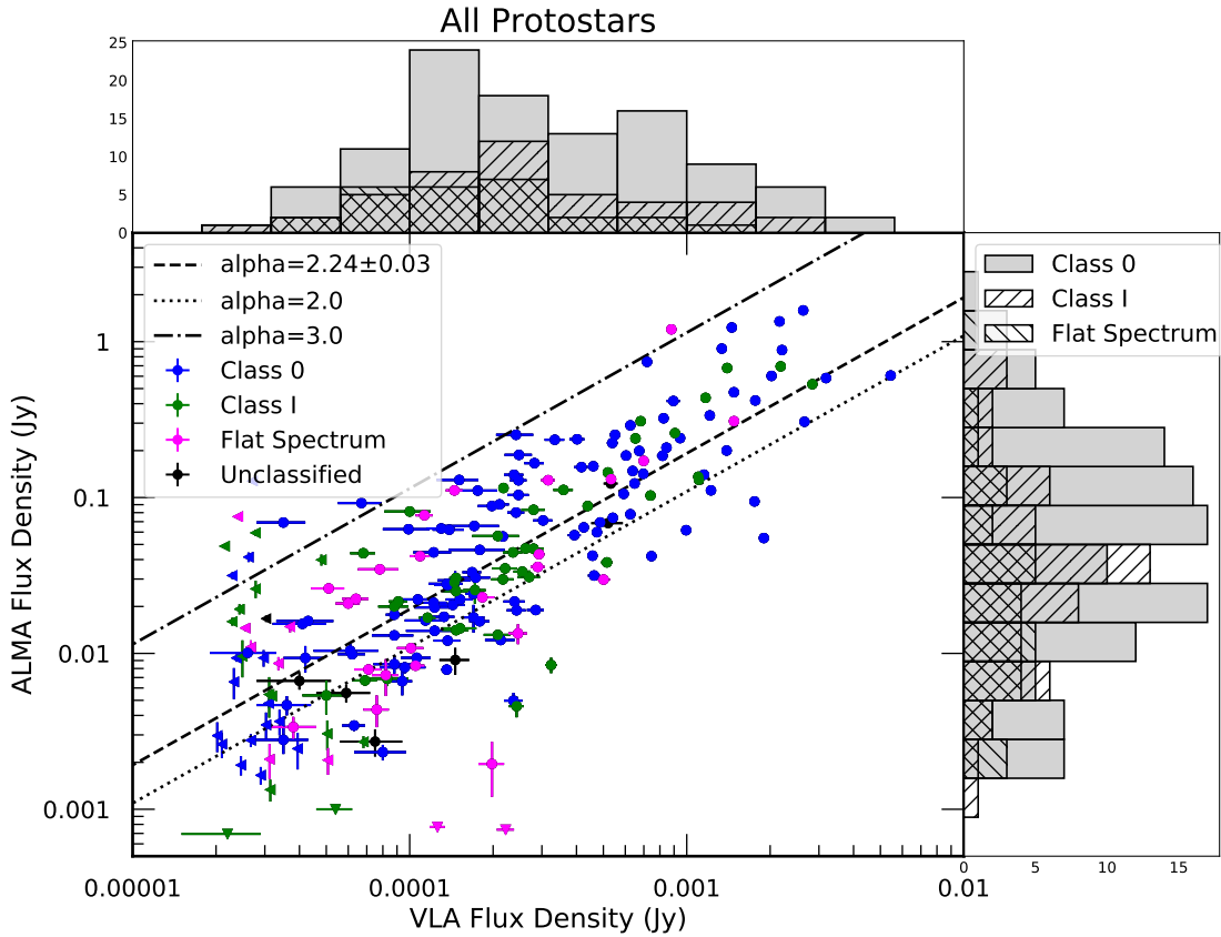
Figure 5. Plot of ALMA 0.87 mm flux density versus VLA 9.1 mm flux density in log-log space. The observational class of the sources are denoted by color where Class 0 protostars are blue, Class I protostars are green, and Flat Spectrum sources are magenta; unclassified sources are black. A strong correlation between the ALMA and VLA flux densities is present, and a constant spectral index can fit the correlation with a spectral index ( \alpha ) \alpha = 2.24 \pm 0.03 (ignoring upper limits). We also plot the line representing \alpha = 2 , points below this line require additional free-free emission to explain their shallow spectral slopes. Most sources have \alpha between 2 and 3, consistent with optically thick to optically thin dust emission. The left pointing or downward pointing triangles denote upper limits for the VLA 9 mm or ALMA 0.87 mm observations, respectively.
