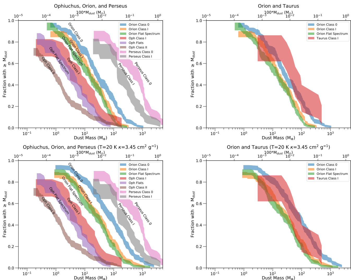
Figure 14. Cumulative distributions of dust disk masses within the Orion sample relative to other protostellar disk surveys; Perseus and Ophiuchus in the left panel and Taurus in the right panel. The top panels use the dust opacity and temperature scaling with luminosity defined in Section 2.4, while the bottom panels use the same dust opacity law as the Ophiuchus/Class II disk samples and a temperature of 20 K. This distribution is for all Orion protostars regardless of multiplicity because the other samples do not exclude multiples. Perseus appears to have higher masses than Orion, but this is likely due to an underestimate of the dust opacity at 9 mm, leading to an overestimate of the masses. The Class I and Flat Spectrum sources from Ophiuchus are significantly lower in mass with respect to Orion. The Class I protostars from Taurus (right panel) are in reasonable agreement with Orion, despite the different methods and small sample.
