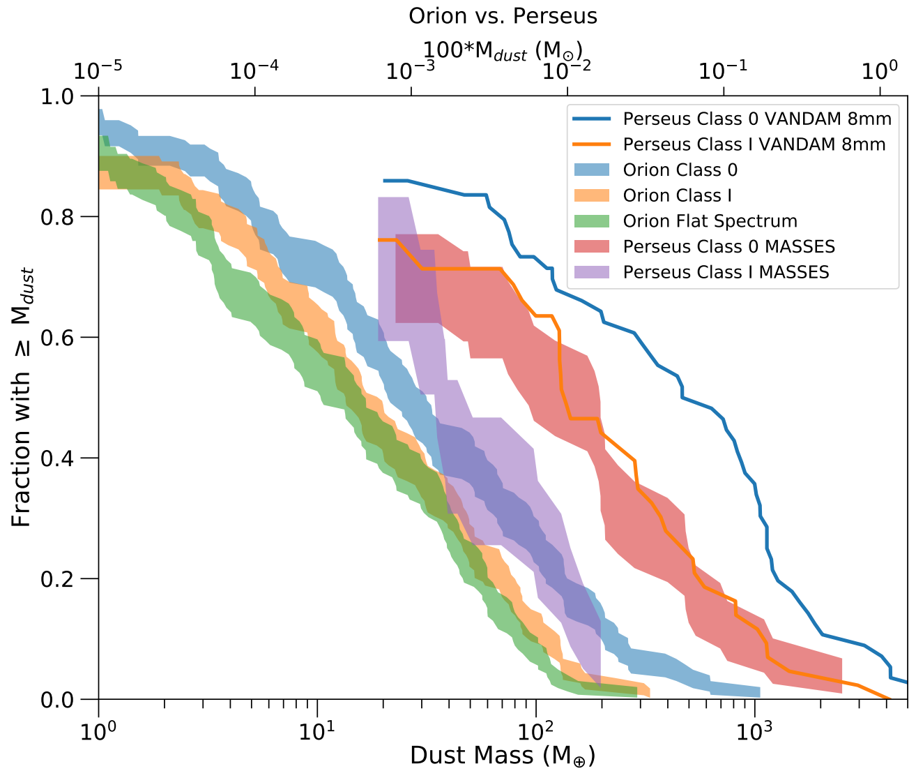
Figure 19. Cumulative distributions of dust disk masses within the full Orion sample relative to the protostellar dust disk mass measurements in Perseus from both VANDAM (Tychoniec et al. 2018) and MASSES (Andersen et al. 2019). The mass distributions from Tychoniec et al. (2018) are drawn as lines in this plot for clarity. This comparison enables us to explore differences that might be due to the wavelengths observed. The values from Andersen et al. (MASSES; 2019) indicate systematically lower masses than those in Tychoniec et al. (VANDAM; 2018), but are still not consistent with the mass distributions of the Orion sample.
