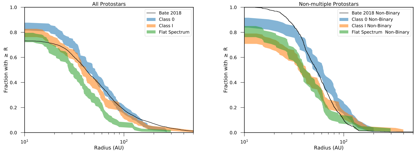
Figure 11. Cumulative distributions of disk radii within the Orion sample. The left panel shows the full sample, while the right panel only shows the non-multiple sample. Protostars with a measured dust disk radius that is \leq 10 au or did not have a measurement due to low S/N is considered an upper limit for the purposes of the survival analysis produced by the lifelines package. Class 0 protostars are drawn with a blue shaded region, Class I protostars are drawn with an orange shaded region, Flat Spectrum sources are drawn with a green shaded region. The Class 0 sources clearly have their distribution shifted toward larger radii; this is more evident in the case of non-multiple sources. The distribution of Class I radii is slightly higher than the Flat spectrum radii for the full sample, but when only considering non-multiple systems, there is very little difference in the distributions. The full sample and non-multiple samples are also compared to the disk radii derived from the large-scale simulations of Bate (2018). The radii distributions from the simulations are comparable to the Class 0 and Class I disk radii for both the full sample and non-multiple cases.
