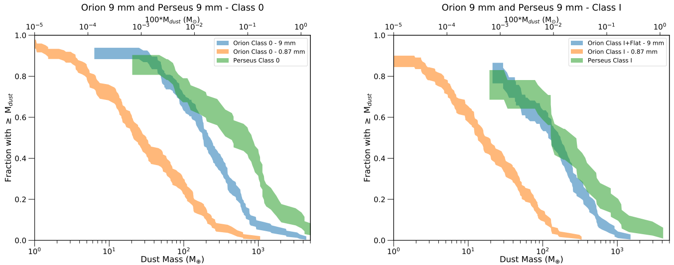
Figure 20. Cumulative distributions of dust disk masses within the Orion sample calculated from 9 mm data compared to the protostellar dust disk mass measurements in Perseus from VANDAM (Tychoniec et al. 2018). The dust disk masses from the Orion 0.87 mm data are also shown for comparison. The Class 0 sources are shown in the left panel and the Class I (combined with Flat Spectrum) in the right panel. Even without the free-free correction to the Orion data, the Class 0 sources from Perseus are still calculated to have higher masses. The Class I sources are more comparable, with some overlap in the distribution.
