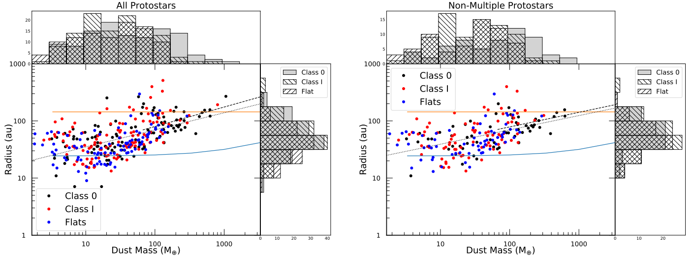
Figure 12. Comparison of disk radii versus dust disk mass for the full sample (left) and the non-multiple sample (right). The Class 0 disks are represented by black points, the Class I disks by red points, and Flat spectrum disks by blue points. There is a clear correlation in that the sources with larger disk radii have higher masses. Smaller disks could have higher masses that cannot be measured due to high optical depth. Upper limits are not shown because an upper limit on disk radius is unphysical if there is not a detection. The solid lines are the analytic prescriptions for disk radii vs. dust disk mass from Hennebelle et al. (2016). The lower line is for the case of disks formed in the presence of magnetic fields, while the upper line is for the case of a disk formed in the hydrodynamic limit; see section 4.6.2. The dotted and dashed lines in the right and left panel are fits to the correlation between radius and mass; the dotted lines only consider masses >33 M_{\oplus} . The relationships are all comparable to R \propto M_{disk}^{0.3} , see Section 3.5 and 4.6.2 for further detail.
