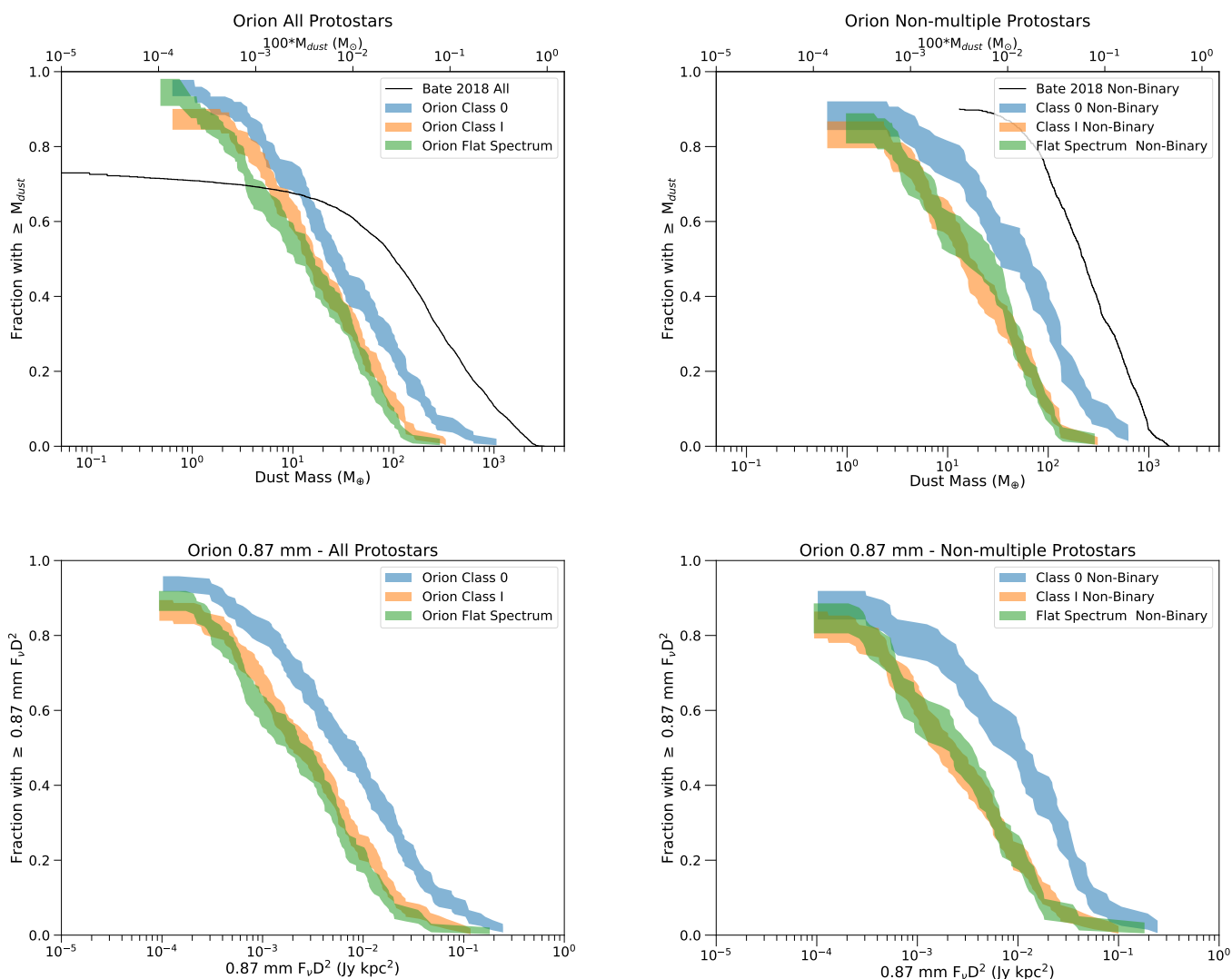
Figure 9. Cumulative distributions of dust disk masses (top row) and 0.87 mm flux densities multiplied by their distance in kpc squared (bottom row) within the Orion sample. The left panels show the full sample, while the right panels only show the non-multiple sample. Class 0 dust disk masses are drawn with a blue shaded region, Class I dust disk masses are drawn with an orange shaded region, Flat Spectrum dust disk masses are drawn with a green shaded region. The Class 0 dust disk masses clearly have their distribution shifted toward higher masses, while there is less difference between the Class I and Flat Spectrum dust disk masses; this is true for the full and non-multiple samples. The full and non-multiple samples are also compared to the dust disk masses derived from the large-scale simulations of Bate (2018). The mass distributions from the simulations have a systematic shift toward higher masses in both the full and non-multiple samples. Statistical comparisons between the dust disk masses of each class is discussed in the text. The distributions of 0.87 mm flux densities, from which the dust disk masses are derived, show the same overall trend of higher 0.87 mm flux densities for Class 0. The Class I 0.87 mm flux densities are systematically higher than Flat Spectrum sources for the population of all protostars, but have substantial overlap for the non-multiple sample.
