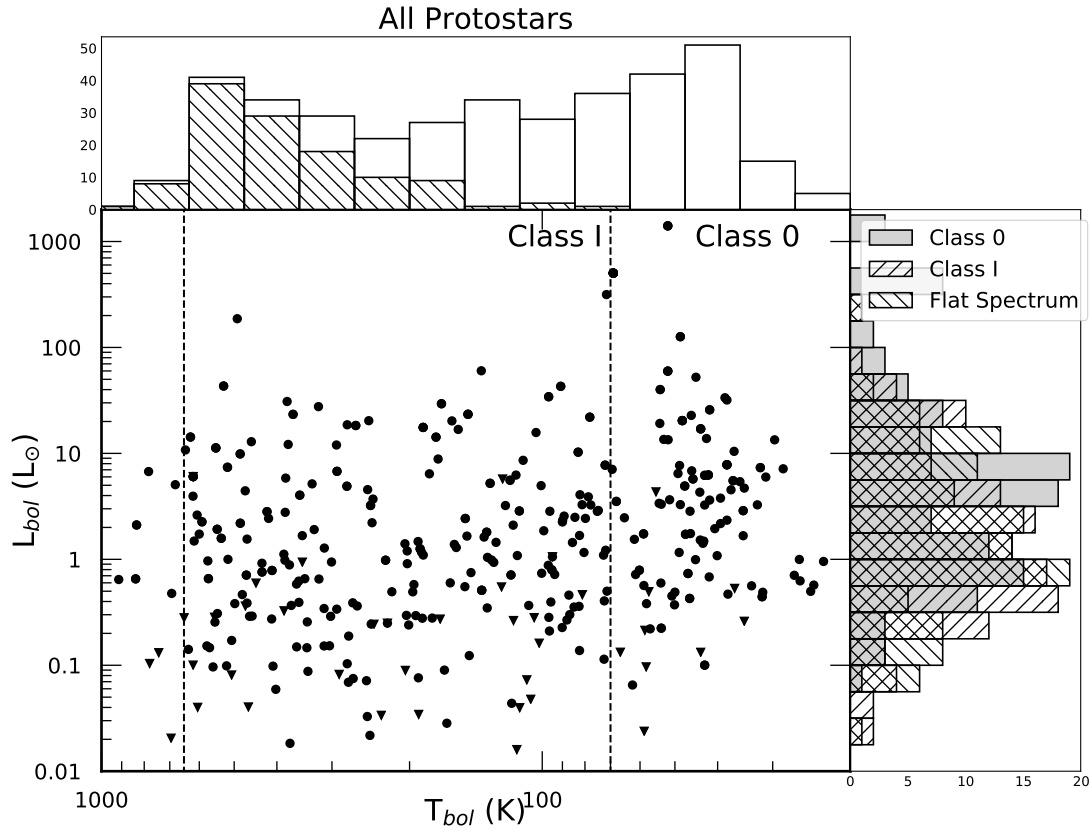
Figure 2. Bolometric luminosity ( L_{bol} ) versus bolometric temperature ( T_{bol} ) for the sample of 328 protostars surveyed by ALMA and the VLA with accompanying histograms. The histogram along the x-axis shows the full number in each bin, and the hatched region shows the number of Flat Spectrum sources, given that they overlap in this parameter space. The histogram along the y-axis shows the distribution bolometric luminosities for each protostellar class in the survey. The distributions are similar, but as shown in Fischer et al. (2017) the Class 0 protostars have slightly higher luminosities on the whole than the Class I and Flat Spectrum protostars.
