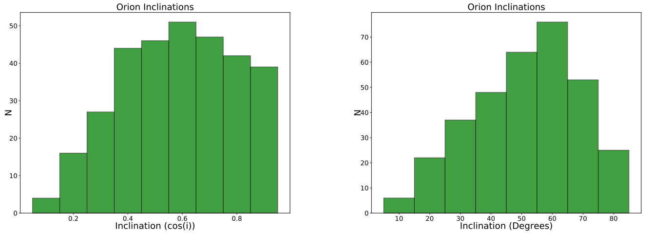
Figure 13. Histogram of inclinations derived from the deconvolved major and minor axes from Gaussian fitting in \cos(i) (left panel) and degrees (right panel). A completely random distribution would be flat in \cos(i) but peaked at 60^\circ . We see that the distribution in \cos(i) starts to drop at values lower than 0.4, which is likely because the deconvolved minor axes fit for sources close to edge-on ( \sim 90^\circ ; \cos(i) = 0 ) are generally overestimated due to the resolution of the survey.
