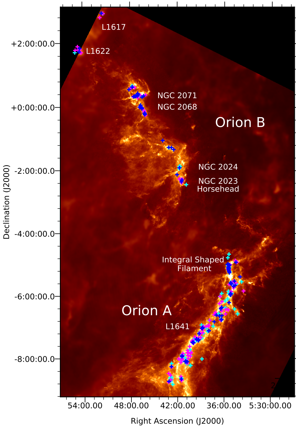
Figure 1. Overview of the Orion region and protostellar targets for the ALMA and VLA surveys (crosses). The image is the Herschel and Planck column density map from Lombardi et al. (2014) displayed on a square-root color scale. Major sub-regions within the clouds are highlighted with the sub-region labels located adjacent to their positions. The blue crosses are Class 0 protostars, magenta crosses are Class I protostars, and cyan crosses are Flat Spectrum protostars.
