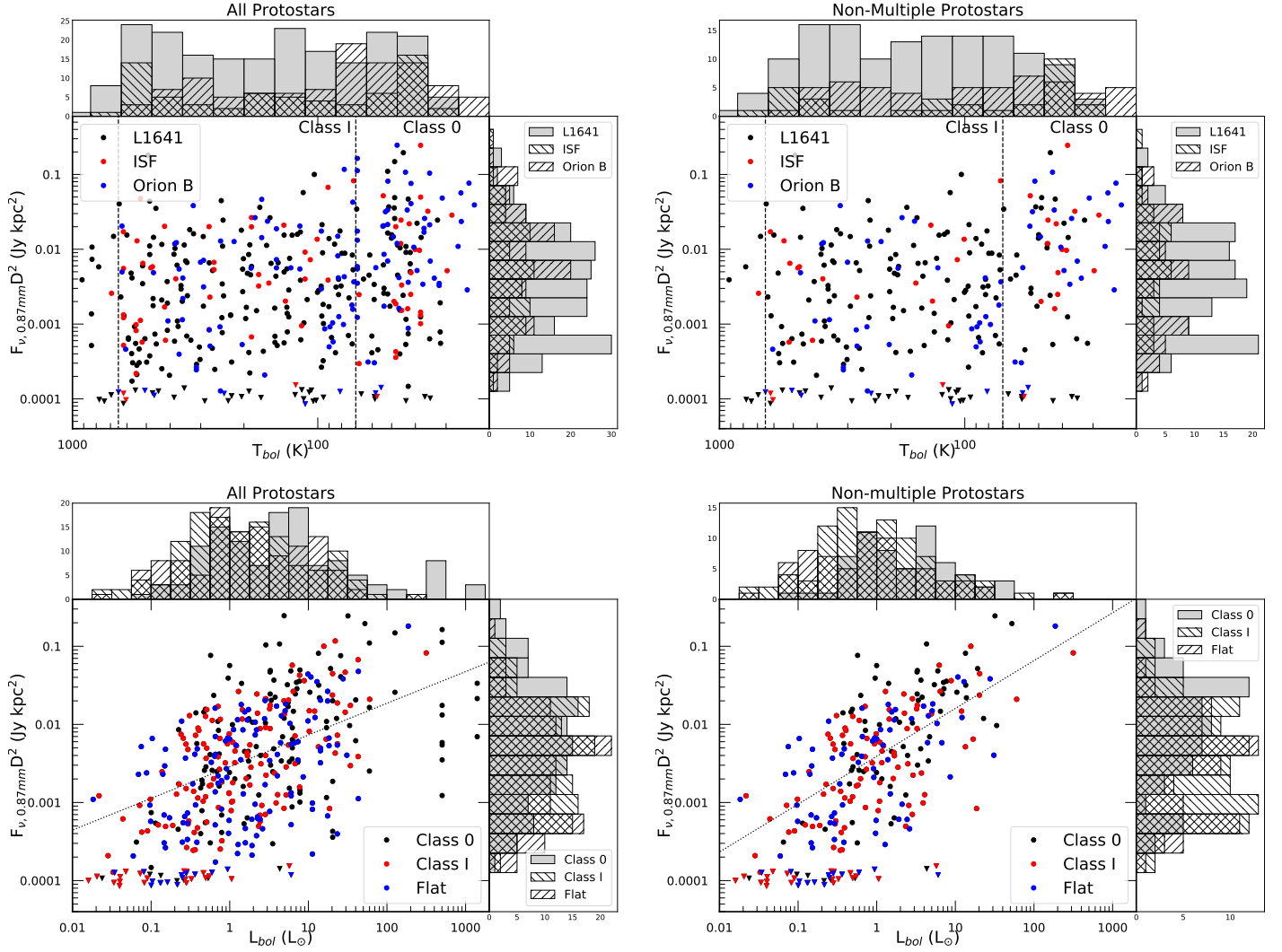
Figure 6. Comparison of 0.87 mm flux densities to T_{bol} (top panels) and L_{bol} (bottom panels); the flux densities are multiplied by the square of their distance in kpc to remove scatter due to different distances within the region. The left panels show the full survey sample with a corresponding measurement of L_{bol} and T_{bol} , while the right panels show only the non-multiple sample. The colorization and histograms associated with the top panels separates the sources by their regions (black: L1641 and southern ISF, red: Northern ISF, blue: Orion B). In the bottom panels, the colors and associated histograms separate the sources by class; black corresponds to Class 0 protostars, red corresponds to Class I protostars, and blue corresponds to Flat spectrum protostars. Upper limits are denoted as downward facing triangles. The lines in the lower panels are the fits to the 0.87 mm flux densities versus L_{bol} , for the full sample (left panel) we find F_{\nu} D^2 \propto L_{bol}^{0.4 \pm 0.04} and for the non-multiple sample (right) we find F_{\nu} D^2 \propto L_{bol}^{0.61 \pm 0.05} . The vertical lines in the top panels denote the separations between Class 0 and Class I (70 K) and Class I and Class II (650 K).
