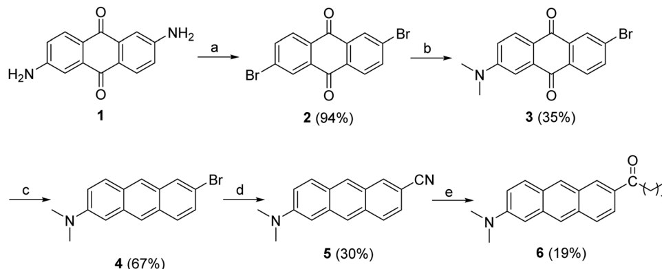
Scheme 1 Reagents and conditions: (a) tert -butylnitrite, \text{CuBr}_2 , \text{CH}_3\text{CN} , 90^\circ\text{C} , 24 h; (b) (1) CsF, DMSO, \text{N}_2 , 170^\circ\text{C} , 5 h; (2) (\text{CH}_3)_2\text{NH} (ac) 40%, \text{K}_2\text{CO}_3 , 70^\circ\text{C} , 17 h; (c) (1) \text{NaBH}_4 , 2-propanol, reflux, 12 h; (2) \text{HCl} (ac) 37%; (d) \text{CuCN} , DMF, \text{N}_2 , reflux 12 h; (e) \text{CH}_3(\text{CH}_2)_6\text{CH}_2\text{MgBr} , \text{CuBr} (cat.), THF, \text{N}_2 , room temperature, 1 h.
