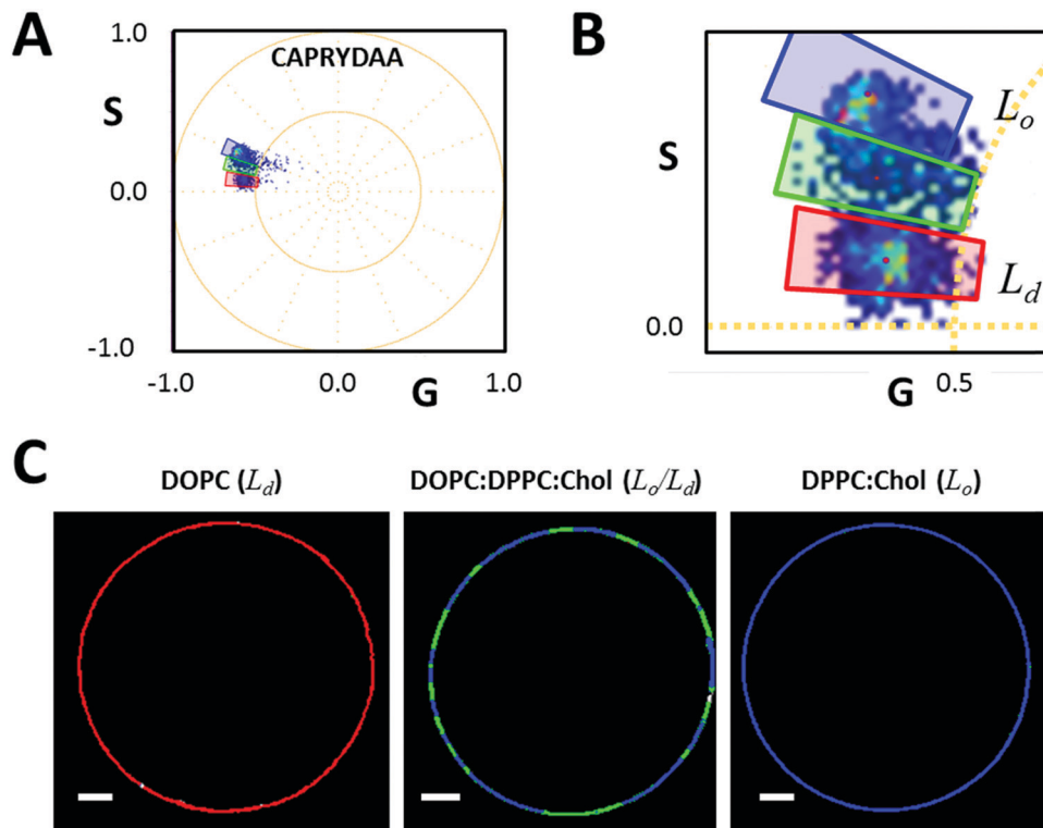
Fig. 7 CAPRYDAA fluorescence in GUVs with different phases. (A) The spectral phasor plot for CAPRYDAA in L_d , L_o , L_d and L_o membranes. (B) Zoom of (A). (C) The representative images of GUVs with L_d , L_o , L_d and L_o phases, respectively.
