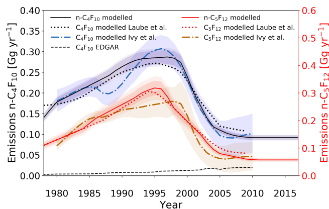
Figure 8. Estimated global emission rates for n -C 4 F 10 and n -C 5 F 12 (full black and red lines, respectively) in this study, global emission rates for C 4 F 10 as reported in the EDGARv4.2 database (dashed black line; no distinction between isomers), modelled emissions by Ivy et al. (2012b) for C 4 F 10 and C 5 F 12 (dash-dotted blue and brown lines, respectively; no distinction between isomers), and modelled emissions by Laube et al. (2012) for C 4 F 10 and C 5 F 12 (dotted black and red lines, respectively; no distinction between isomers). Note that the maximum EDGARv4.2 emission rate for n -C 5 F 12 is less than 0.6 \times 10^{-4} and is therefore not plotted here. Shadings illustrate the uncertainties.
