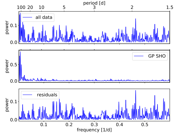
Figure F2. Periodogram of H\alpha data (top), of the SHO kernel (middle) and of the residuals (bottom).
