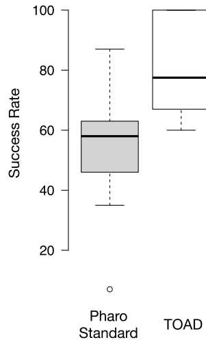
Fig. 5. Extract Method Success Rate.
