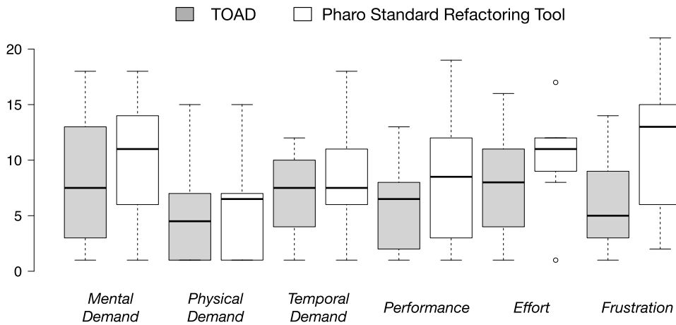
Fig. 6. Task Load: Participant Perceptions.
