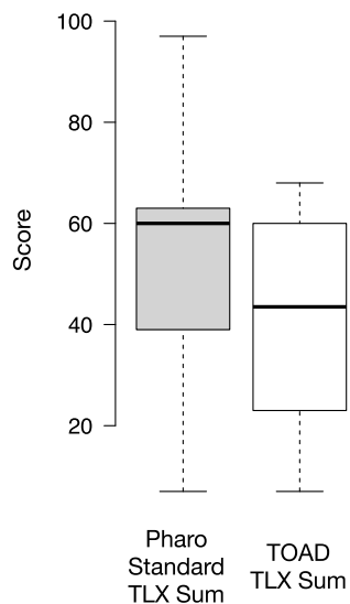
Fig. 7. Total cognitive load (lower is better).
