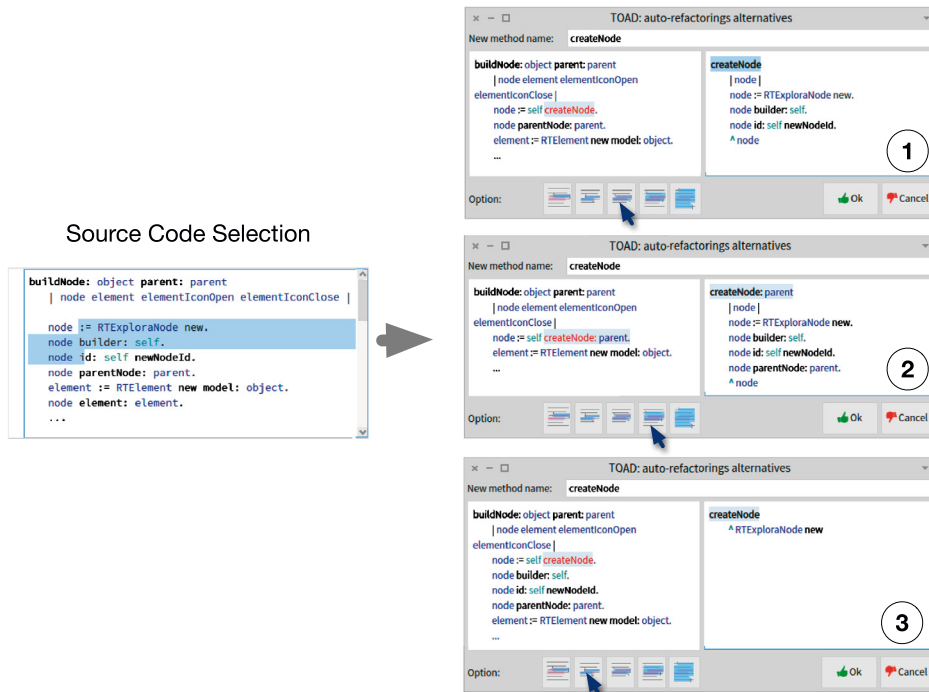
Fig. 4. TOAD in action: five adequate selections are suggested from an invalid selection made by a user. The figure shows three of these suggestions.
