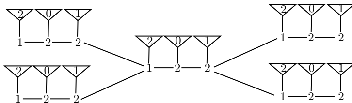
Fig. 6: Gadget of OR gates used in the graph shown in Figure 4. Signals are transmitted and coded based on the block gadget.
