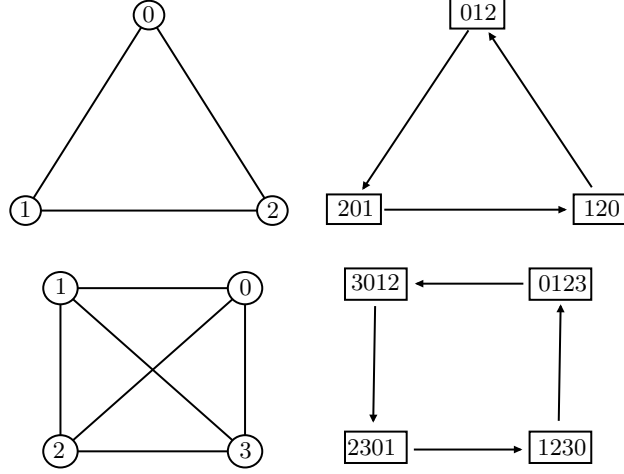
Fig. 1: Attractors with period p = \tau + 1 for \tau = 2 and \tau = 3 . a) Conjunctive network with firing memory and delay dt_i = 2 in every node that admits a limit cycle with period 3. On the left hand side we show the interaction graph of the network and on the right hand side there is the transitions graph of the cycle. b) Conjunctive network with firing memory and delay dt_i = 3 in every node that admits a limit cycle with period 4. On the left hand side we show the interaction graph of the network and on the right hand side there is the transitions graph of the cycle.
