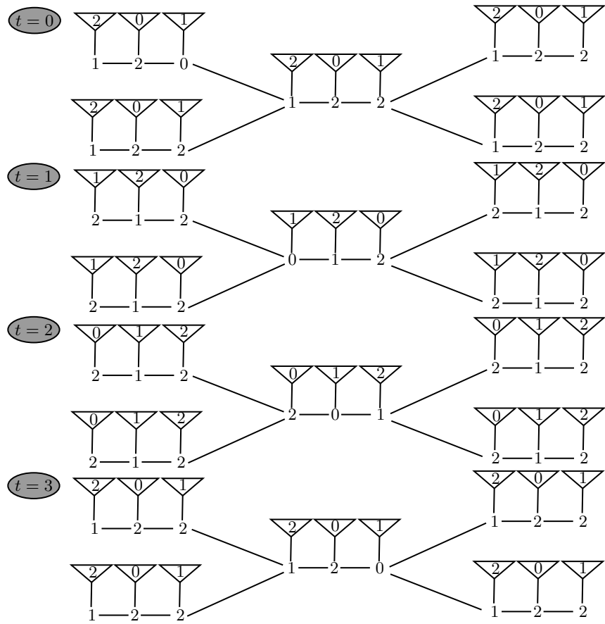
Fig. 13: Iterations of the OR gate gadget. A 0 and a 1 are computed as inputs. After three steps the information is transmitted and the initial condition is recovered.
