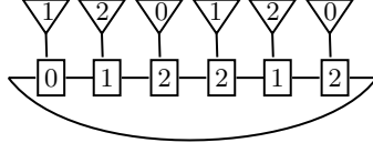
Fig. 10: An interaction graph G associated to a conjunctive network with firing memory and maximum delay values dt_i = 2 for all i \in V(G) that admits attractors with period 6. Every triangle represents a conjunctive network with firing memory that admits attractors with period 3 and states in the triangles represent the states of the nodes that are connected to the nodes in the path.
