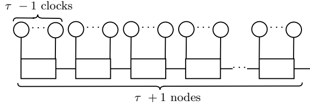
Fig. 3: Structure of a block used in Proposition 2 (see Appendix Section A.1, Proposition 1 for the complete proof) to define a conjunctive network with firing memory and maximum delay values dt_i = \tau for every node i that admits attractors with period k(\tau + 1) . Every circle in the figure represents clock associated to a node r represented by a square. This gadget has \tau + 1 nodes and every node has \tau - 1 clocks.
