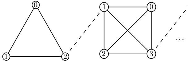
Fig. 2: A construction of a conjunctive network with firing memory which admits attractors of non polynomial period. The interaction graph is a connected union of complete graphs K_{p_i+1} with p_i a prime number. Each component is setted to an initial condition according to Proposition 2 and the connections between components are arbitrary. Global initial condition x is defined such that nodes in initial state 0 are not allowed to be connected.
