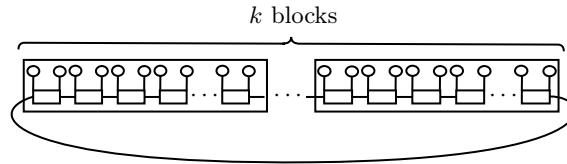
Fig. 9: Interaction graph G associated to a conjunctive network with firing memory and maximum delay dt_i = \tau for all i \in V(G) , defined in Proposition 2 that admits attractors with length k(\tau + 1) .
