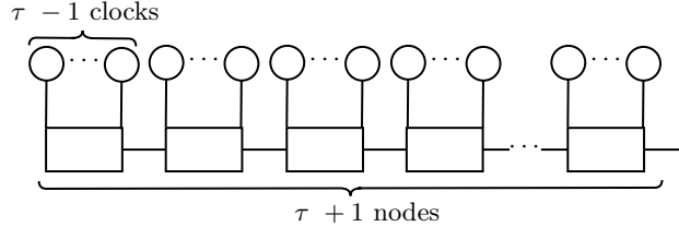
Fig. 7: Structure of the j -th block used in Proposition 2 to define a conjunctive network with firing memory and maximum delay values dt_i = \tau for every node i that admits attractors with period k(\tau + 1) . Every circle in the figure represents clock C(B_j)_{r,l} associated to a node r represented by a square. This gadget has \tau + 1 nodes and every node has \tau - 1 clocks.
