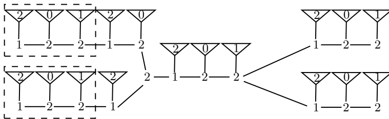
Fig. 5: Gadget of AND gates used in the graph shown in Figure 4. Signals are transmitted and coded based on the block gadget.
