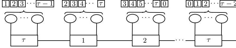
Fig. 8: Initial condition for the j -th block, j \geq 2 used in Proposition 2 to define an attractor with period k(\tau + 1) . For the first block we just define the state of the first node to 0 instead of \tau .
