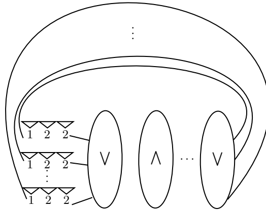
Fig. 4: Interaction graph associated to a conjunctive network with firing memory and maximum delay vector dt_i = 2 for every node i that simulates an iterated monotone boolean circuit C . Layers are made up by AND or OR gates exclusively, using the gadgets shown in Figure 5 and Figure 6 are alternately ordered.
