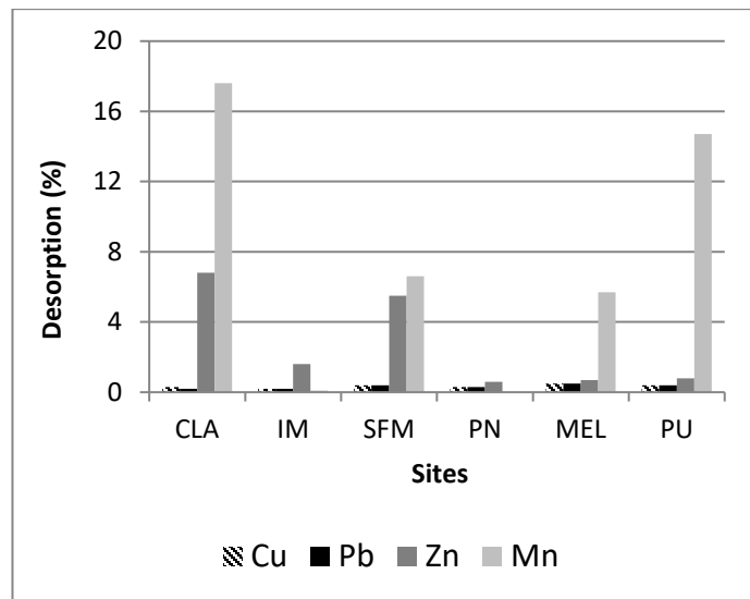
Figure 4. Concentration (%) of metals desorbed since sediments
