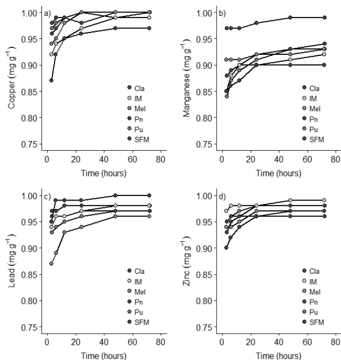
Figure 2. Curves of adsorbed metal Cu (a); Mn (b); Pb (c) and Zn (d) ( \text{mg g}^{-1} ) as a function of contact time (hours) onto sediment of the six sites in the Maipo River basin.
