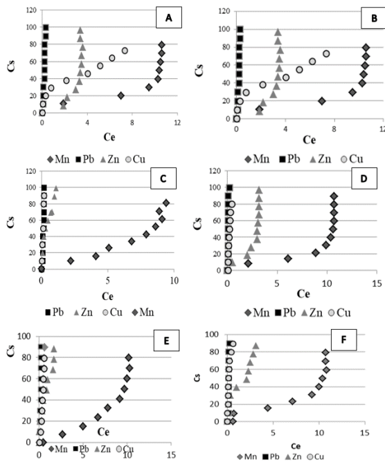
Figure 3. Adsorption isotherms of metals Cu, Mn, Pb and Zn. a) CLA (b) IM (c) MEL, d) PN (e) PU (f) SFM. Cs = adsorption concentration (mgL -1 ); Ce = concentrations in solution (mgL -1 ).
