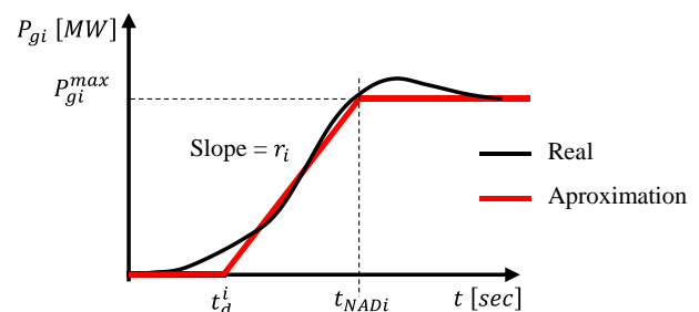
FIGURE 2. Dynamic response of a synchronous generator during a power imbalance [52] and adopted approximation.
