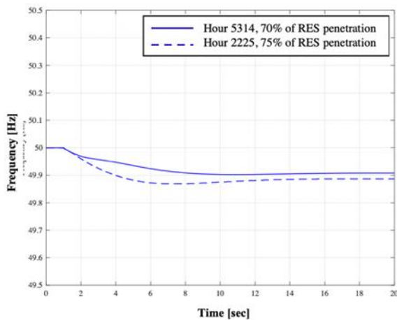
FIGURE 7. Frequency evolution after the loss of the largest SG in operation in hour 5314 (91 MW) and in hour 2225 (89 MW).
