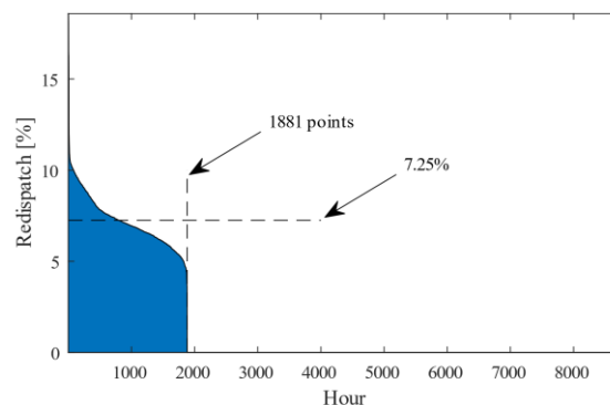
FIGURE 5. Duration curve of the percent redispatched power .
