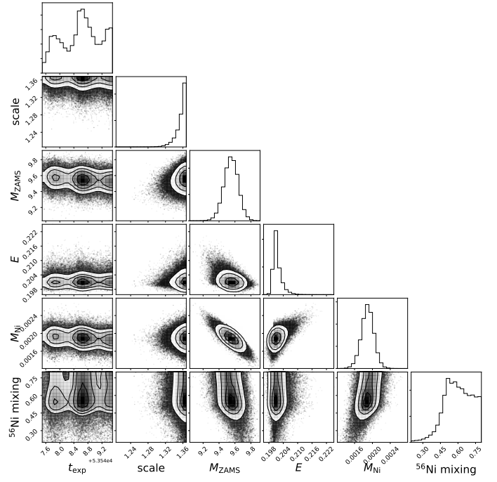
Fig. A.4. Same as for Fig. 4 but for SN 2005cs.
