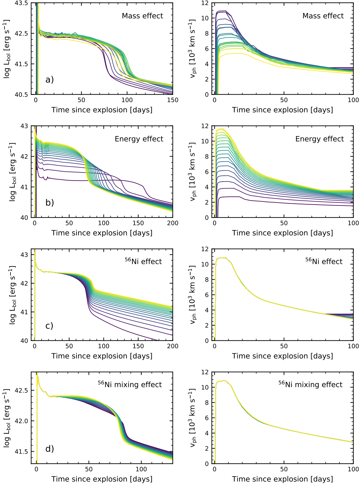
Fig. A.1. Interpolated synthetic bolometric LCs (left panels) and photospheric velocities (right panels) after varying the progenitor initial mass between 9 and 25 M_{\odot} (panel a), the explosion energy between 0.1 and 1.5 foe (panel b), the 56 Ni mass between 0.005 and 0.08 M_{\odot} (panel c), and the 56 Ni mixing between the 20% and 80% of the final structure in mass coordinate (panel d). The values increase from purple to yellow. Eighteen models are shown for each parameter been varied. The parameters not being varied are fixed at an initial mass of 10 M_{\odot} , explosion energy of 1.3 foe, M_{\text{Ni}} of 0.01 M_{\odot} , and 50% of 56 Ni mixing, with the exception of the panel showing the 56 Ni mixing effect for which a larger M_{\text{Ni}} of 0.06 M_{\odot} is used to enable better visualisation of this effect.
