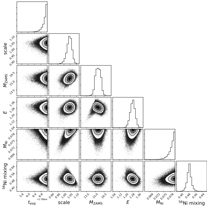
Fig. A.7. Same as for Fig. 4 but for SN 2017eaw.
