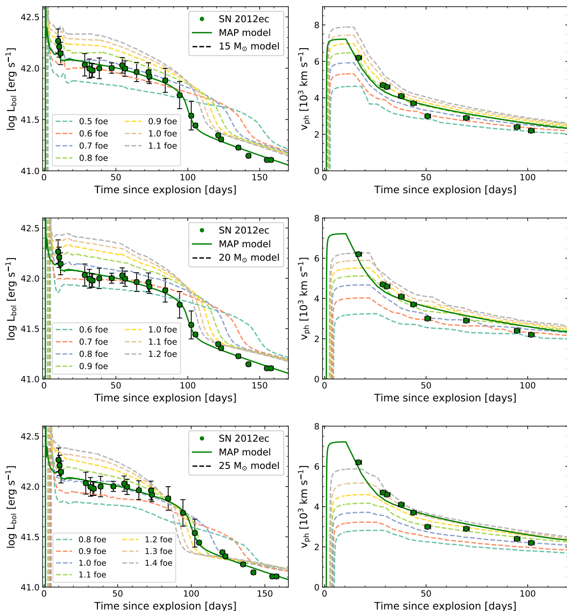
Fig. 11. Hydrodynamic models for different M_{\text{ZAMS}} (dashed lines) compared to the MAP model (solid line) and observations of SN 2012ec (green dots). Dashed lines are colour-coded according to different explosion energy. The models plotted correspond to the same values of M_{\text{Ni}} and ^{56}\text{Ni} mixing as the MAP model. The MAP model is reproduced with M_{\text{ZAMS}} = 9.9 M_{\odot} , E = 0.57 foe, M_{\text{Ni}} = 0.034 M_{\odot} , and ^{56}\text{Ni} mixing = 28%. Left panels: bolometric LCs. Right panels: evolution of the photospheric velocity. Top panel: 15 M_{\odot} model. Middle panel: 20 M_{\odot} model. Bottom panel: 25 M_{\odot} model.
