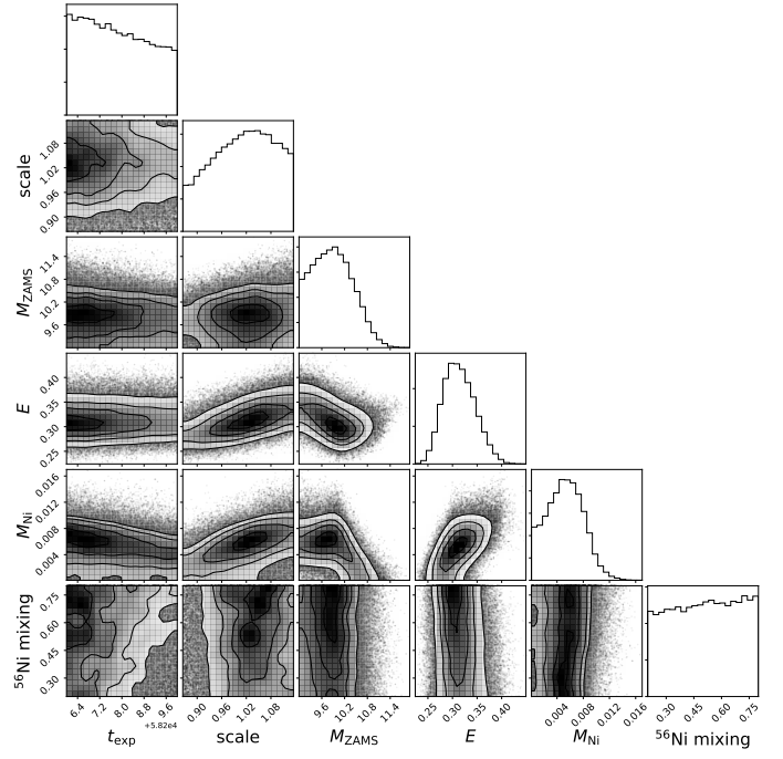
Fig. A.8. Same as for Fig. 4 but for SN 2018aoq.
