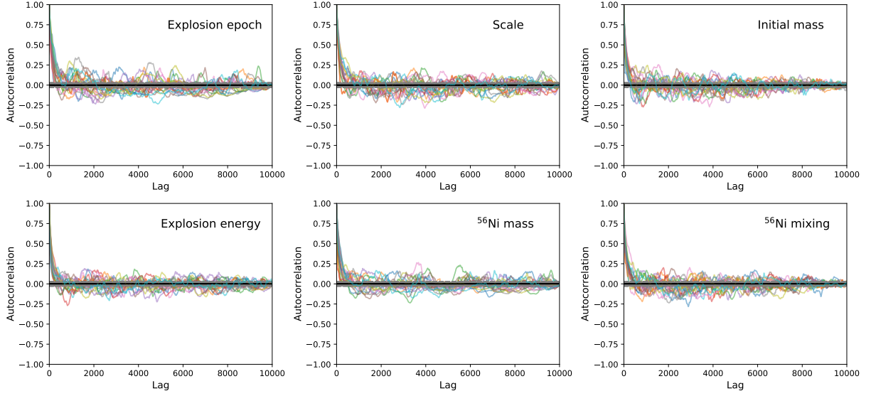
Fig. A.10. Autocorrelation plots for twenty chains randomly chosen using SN 2017eaw as example. Each panel shows the autocorrelation for a different parameter.
