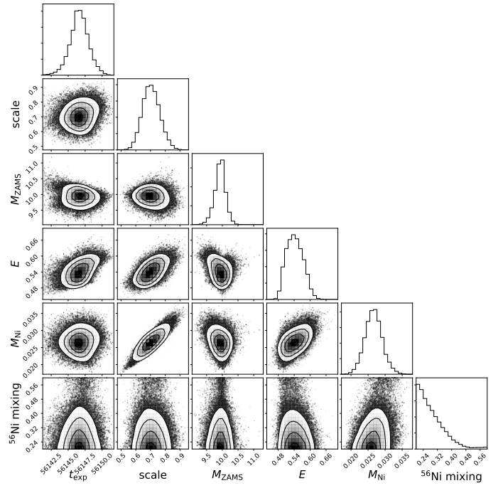
Fig. A.9. Corner plot of the joint posterior probability distribution of the parameters for SN 2012ec when the priors for t_{\text{exp}} and the scale are relaxed.
