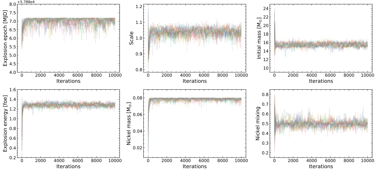
Fig. A.11. Trace plots of the parameters for twenty chains randomly chosen using SN 2017eaw as example. These plots show the evolution of the chains over time.
