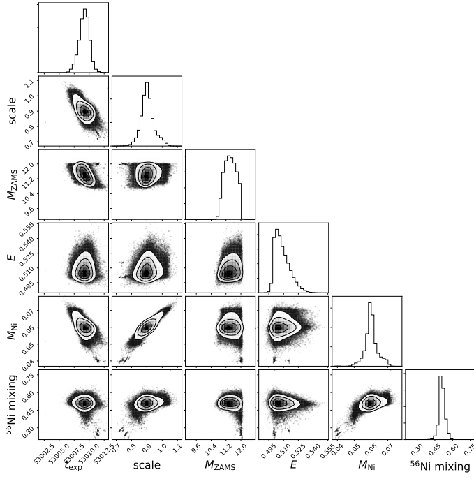
Fig. A.2. Same as for Fig. 4 but for SN 2004A.
