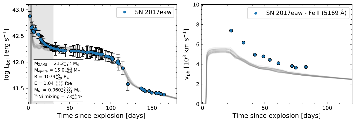
Fig. 12. Bolometric LC (left panel) and photospheric velocity evolution (right panel) for SN 2017eaw in comparison with fifty hydrodynamical models randomly chosen from the posterior probability distribution. In this example we did not take into account the photospheric velocity for the fitting. We can note the importance of fitting both observables simultaneously.
