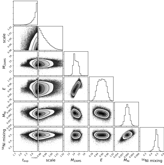
Fig. A.6. Same as for Fig. 4 but for SN 2012aw.
