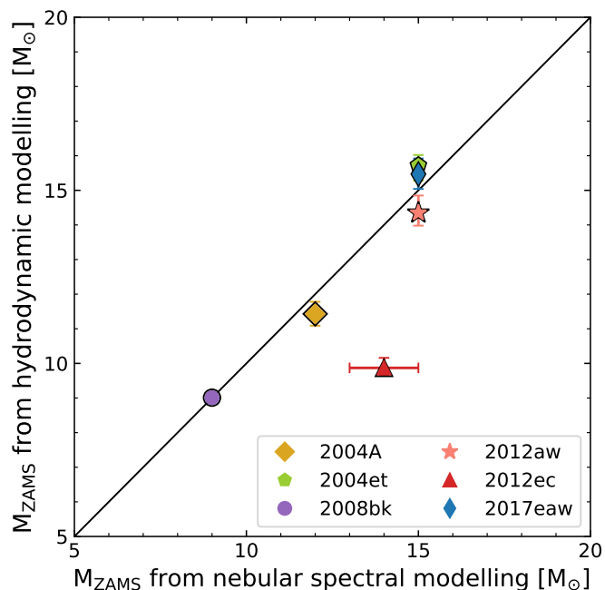
Fig. 8. Comparison between M_{ZAMS} obtained from hydrodynamic and late-time spectral modelling. An excellent agreement can be seen for all SNe II except SN 2012ec.
