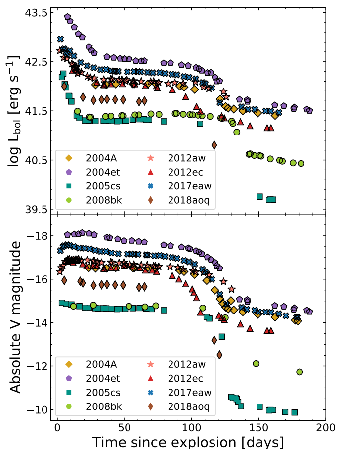
Fig. 3. Bolometric LCs (top panel) and absolute V -band LCs (bottom panel) of SN 2017eaw and SN 2018aoq in comparison with the well-studied SN 2004A, SN 2004et, SN 2005cs, SN 2008bk, SN 2012ec, and SN 2012aw. Absolute curves were computed using the distances and reddenings in Table 1 of MB19, except SN 2004et for which we use the new estimates of the distance (see text).
