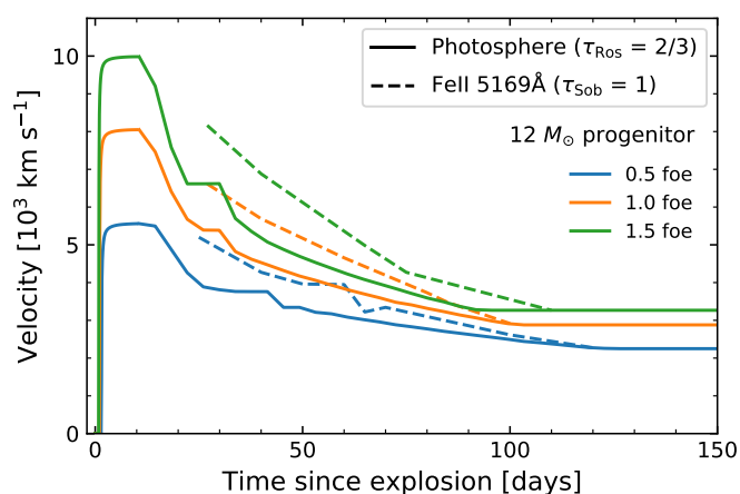
Fig. 14. Comparison of the photospheric velocity and the Fe II line velocity for a 12 M_{\odot} progenitor and different explosion energies.
