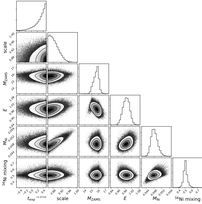
Fig. A.3. Same as for Fig. 4 but for SN 2004et.
