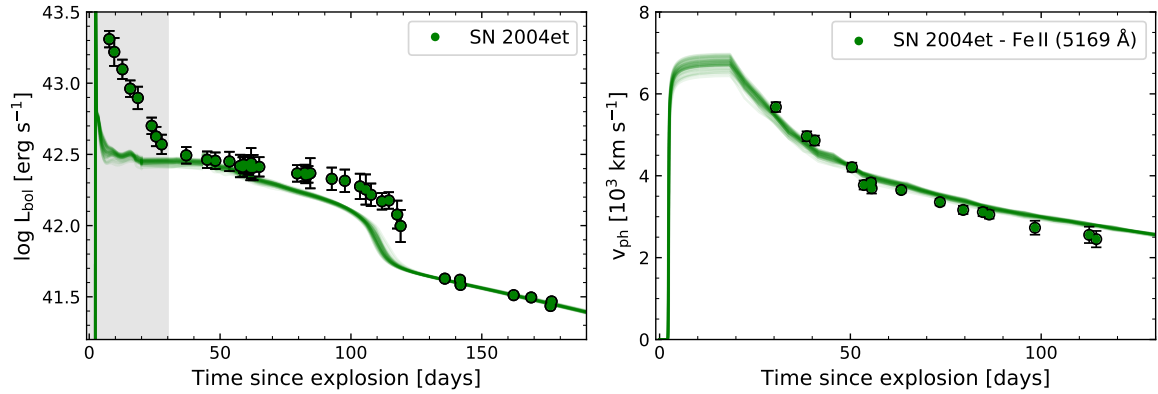
Fig. A.12. Comparison between models and observations for SN 2004et assuming d = 7.73 \pm 0.78 Mpc. We show fifty models randomly chosen from the posterior probability distribution. The lack of agreement during the photospheric phase is easily seen. Left: bolometric LC. Right: evolution of the photospheric velocity. The grey shaded region shows the early data we removed from the fitting.
