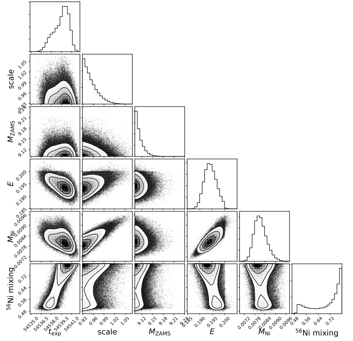
Fig. A.5. Same as for Fig. 4 but for SN 2008bk.
