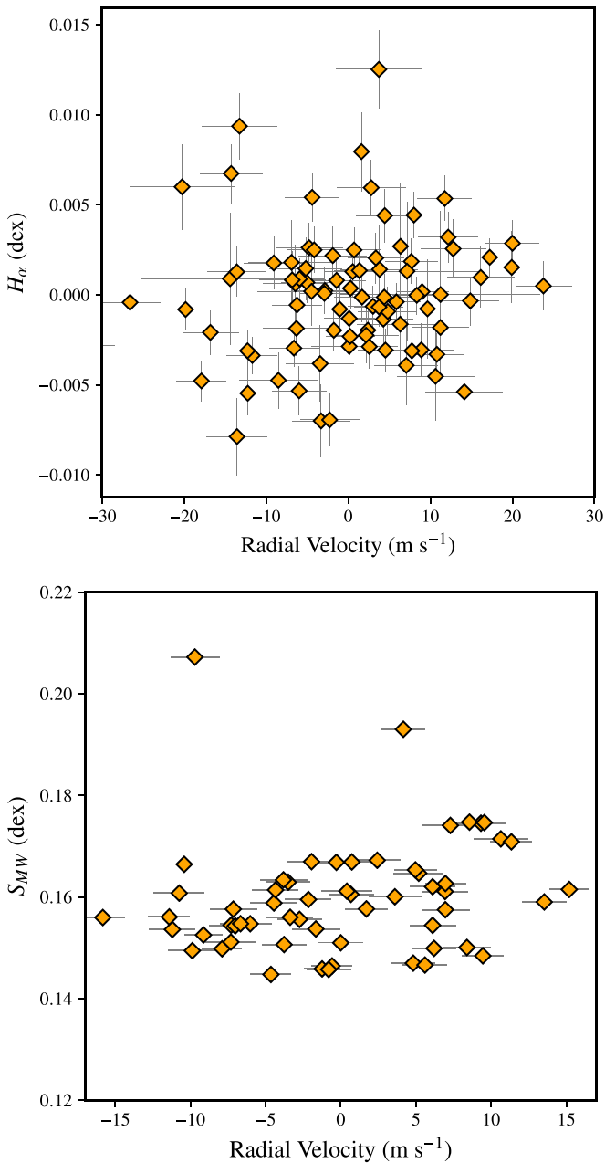
Figure 12. Top: Correlations between RVs and H_{\alpha} index from CORALIE. Bottom: Correlations between RVs and S-index ( S_{MW} ) values from PFS. On each plot, we have subtracted the mean value of both Rv and the activity indices.
