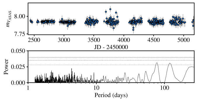
Figure 3. GLS periodogram of the ASAS V -band photometry. Dashed lines from top to bottom represent the 0.1, 1 and 10% significance threshold levels, respectively, obtained via 10,000 bootstraps samples.
