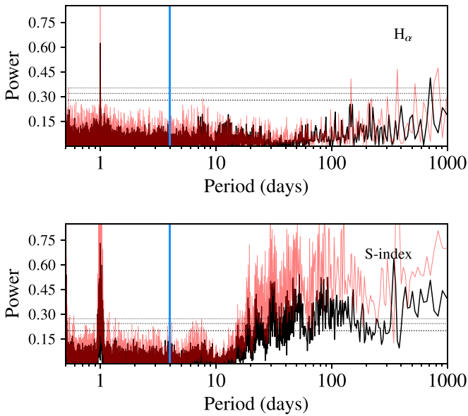
Figure 7. Top: GLS periodogram for H_{\alpha} indices from CORALIE. Bottom: Generalized L–S periodogram of S-indices from PFS. In both panels, the blue vertical line represents the position of the 3.9 day period of the planet candidate. Red power spectra show the window function.
