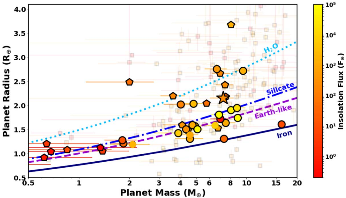
Figure 11. Visualization of where HD 86226c (bold-outlined star symbol) falls among other detected planets in terms of its mass and radius. Circle symbols correspond to planets with errors in radius and mass similar to those of HD 86226c ( \sigma_{R_p} \leq 0.1 R_\oplus and \sigma_{M_p} \leq 1.2 M_\oplus errors), with masses measured via RV observations. Pentagon symbols correspond to planets with the same \sigma_{R_p} and \sigma_{M_p} limits, but with masses measured via transit-timing observations. Bold-outlined circles and pentagons correspond to multiplanet systems. Fainter background squares correspond to the remaining planets with lower-precision mass and radius measurements from either RV or TTV observations. Colored curves represent estimates of different bulk compositions—H 2 O (light blue dotted), silicate (dark blue dashed-dotted, no iron), Earth-like (purple dash), and pure iron (dark blue solid). See Section 6.1 for details on the interior modeling.
