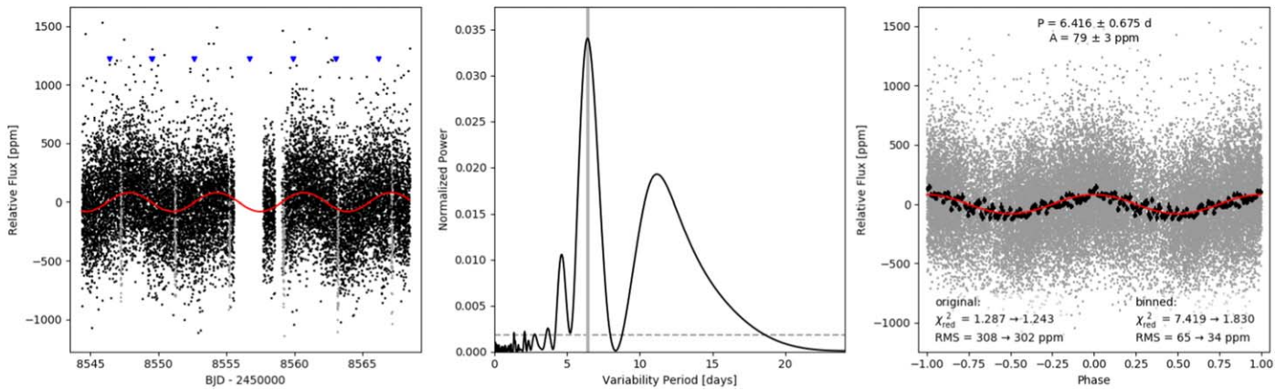
Figure 1. TESS photometric variability. Left panel: PDC lightcurve with transits masked (gray) and reaction wheel desaturation events marked with blue triangles. Middle panel: L–S periodogram with the strongest peak at 6.4 days marked with a vertical gray line. Horizontal dashed line represents a FAP of 0.01. Right panel: Phase-folded lightcurve at the variability period, with (black) and without binning (gray). Best-fitting variability function is shown in red.
