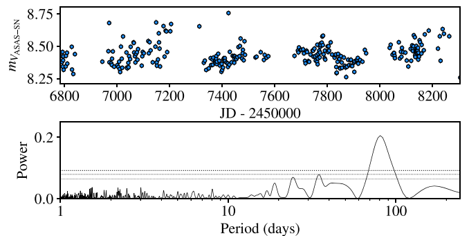
Figure 4. GLS periodogram of the ASAS-SN V -band photometry. Dashed lines from top to bottom represent the 0.1, 1 and 10% significance threshold levels, respectively, obtained via 10,000 bootstrap samples.
