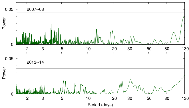
Figure 5. Periodogram of the WASP-South data from the 200 mm lenses (top) and 85 mm lenses (bottom). Horizontal lines are the estimated 1% false-alarm levels.
