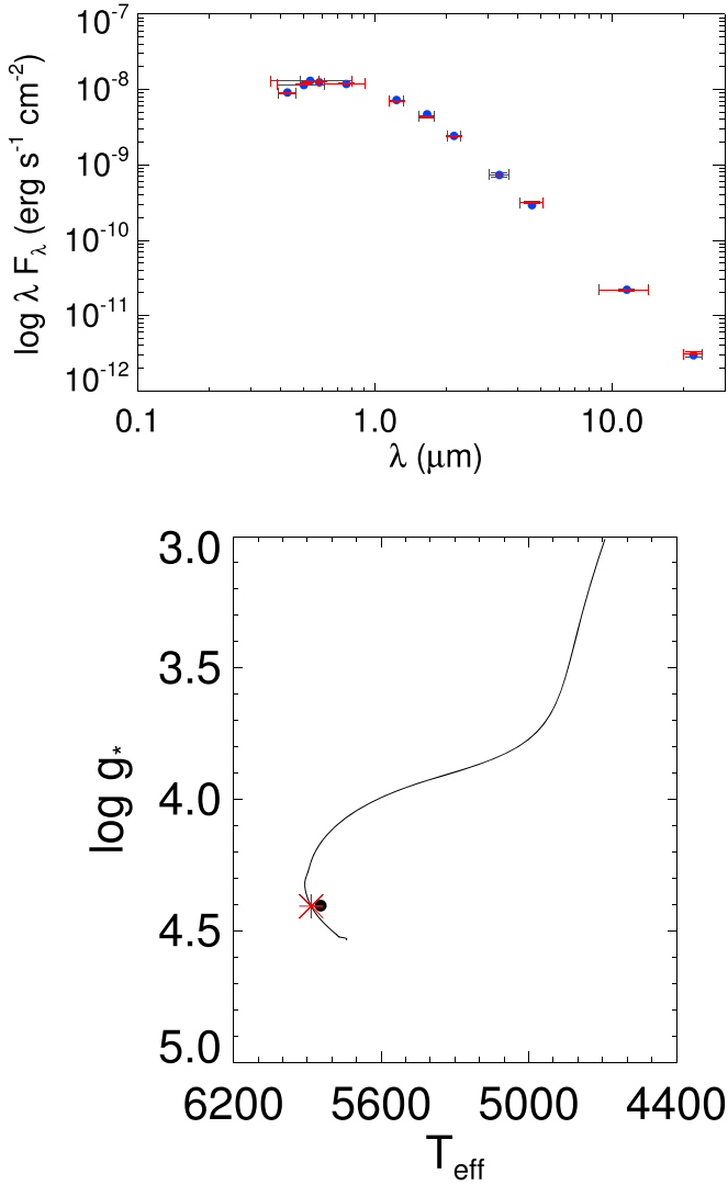
Figure 8. SED (top, see Table 4) and fit to MIST stellar evolutionary model (bottom) for HD 86226. Resulting parameters are listed in Table 5.
