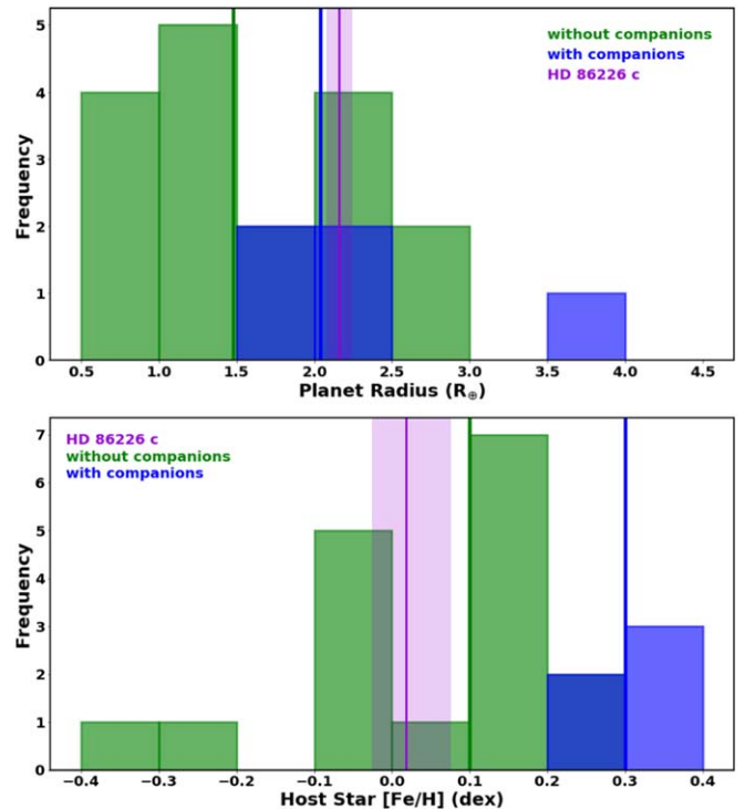
Figure 14. Comparison of HD 86226c (purple, with shading corresponding to 1\sigma errors) to planets within \pm 2\sigma of its mass from the B19 sample. Top: Green histogram (vertical line) represents the distribution (median) of the radii of planets without giant planet companions. Blue histogram (vertical line) represents the distribution (median) of the radii of planets with giant planet companions. Bottom: Green histogram (vertical line) represents the distribution (median) of the host star metallicities of planets without giant planet companions. Blue histogram (vertical line) represents the distribution (median) of the host star metallicities of planets with giant planet companions.
