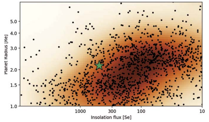
Figure 13. Insolation flux relative to Earth as a function of planet radius, extracted from the NASA Exoplanet Archive. Data are presented in a fashion similar to that in Fulton et al. (2017) and Fulton & Petigura (2018). Shading represents point density, showing the different populations of sub-Neptunes and super-Earths, with dense populations shown in darker shades. Light area in the upper left of the plot indicates the hot Neptune desert. HD 86226c is shown as a green star toward the edge of the desert.
