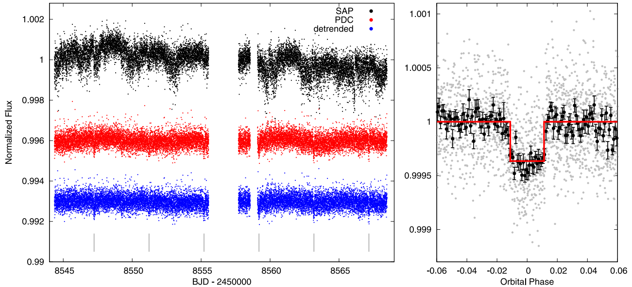
Figure 2. TESS lightcurve of HD 86226 and our preliminary transit detection. Left panel shows the simple-aperture (SAP, top, black), systematics-corrected (PDC, middle, red), and detrended (bottom, blue) TESS photometry, with the transits of TOI-652.01 (HD 86226c) marked with gray vertical lines at the bottom of the panel. Right panel shows the detrended lightcurve in gray, and in phase bins of 0.001 in black, folded to the period of TOI-652.01 as identified by the BLS periodogram. Detected transit is shown as a red line in the right panel.
