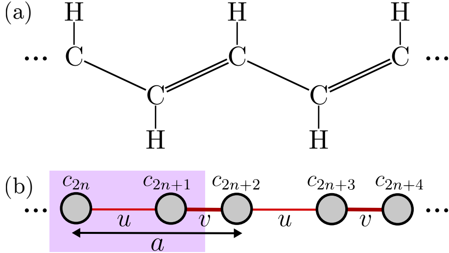
FIGURE 1.2: (a) Chemical scheme of polyacetylene. (b) Scheme of the tight binding SSH model. Sites are represented by grey circles and hoppings by red lines. The unit cell is highlighted in purple, and the lattice periodicity constant a is shown over the lattice.
