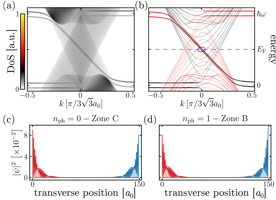
FIGURE 4.3: (a) Density of States (DoS) near the edges of a semi-infinite zigzag ribbon, in arbitrary units. A valley selective gap opens in the replica crossing, bridged by two edge states with parallel velocities. These states coexist with a continuum of extended states of the ungapped valleys. (b) Band structure of a zigzag ribbon (of width 150a_0 ). The color scale indicates the weight of the bands on n_{\text{ph}} = 0 (black) and n_{\text{ph}} = 1 (red), while the transparency of the curves is related to the localization of the states (ranging from light curves for extended states, to opaque curves for states with an inverse participation ratio larger than 0.1). The edge states described in (a), at energy E_F = \hbar\omega/2 , are indicated with a blue circle. The horizontal axis in (a) and (b) corresponds to the rBZ projected to the periodicity direction. (c) and (d) Projection of the edge states in (b) to zone C of the BZ in n_{\text{ph}} = 0 , and zone B in n_{\text{ph}} = 1 , showing that they are localized at opposite borders of the ribbon. Other parameters used are \gamma_1 = 0.025\gamma_0 , \hbar\omega = 0.3\gamma_0 , and \Delta = 0.01\gamma_0 .
