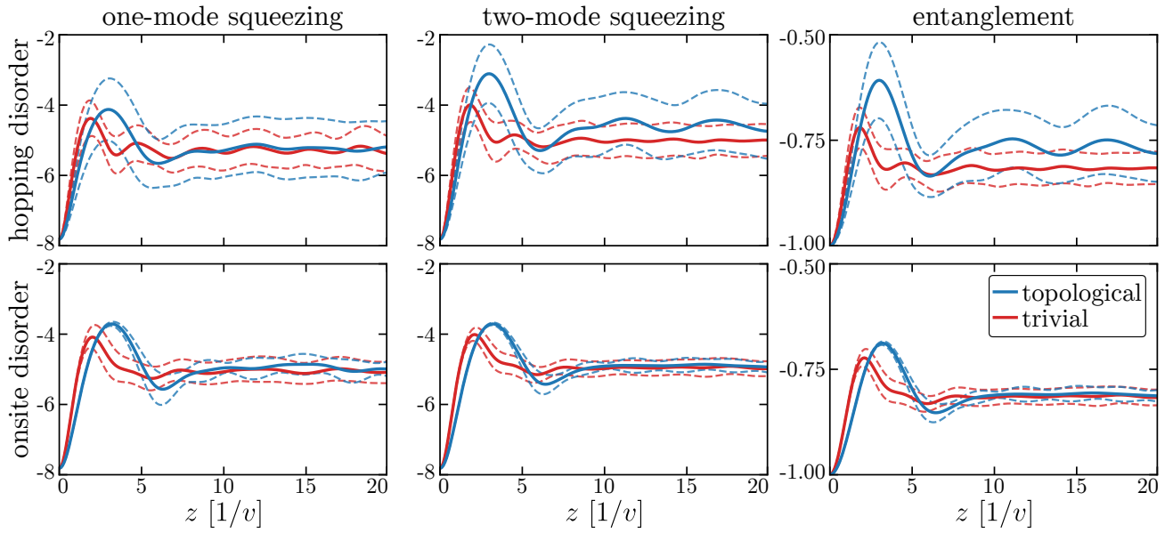
FIGURE B.1: Maximal one-mode squeezing corresponding to the data in Fig. 3.4, and maximal two-mode squeezing and entanglement corresponding to the data un Fig. 3.5. Statistical average values are represented by solid lines, while dashed lines represent the confidence interval associated with the standard deviation, with blue (red) lines referring to the topological (trivial) system.
