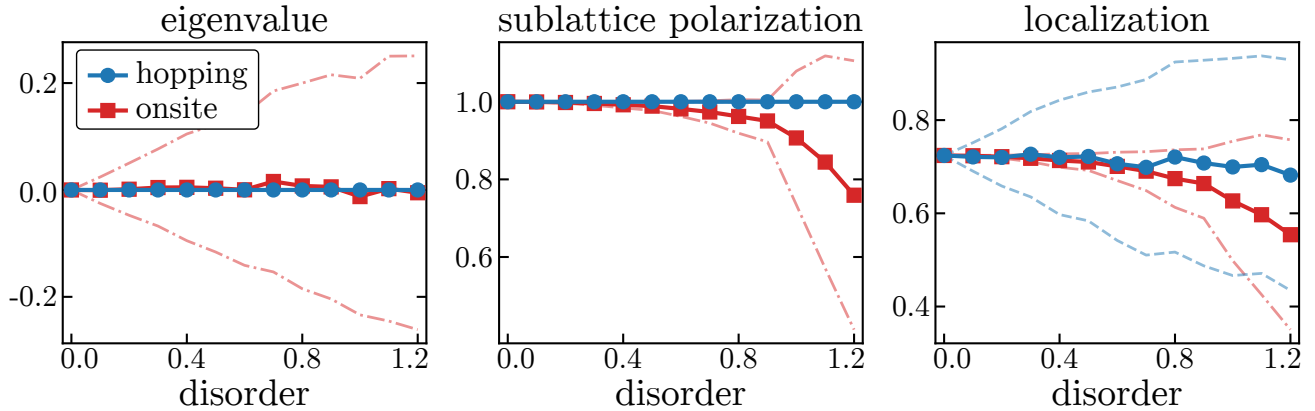
FIGURE 1.5: Eigenvalue, sublattice polarization and localization of the edge state of a semi-infinite SSH lattice in presence of random hopping and onsite disorder, for u = 0.4 and v = 1 . Solid lines with marker show average value, while dashed lines show standard deviation. Sublattice polarization of state |\chi\rangle is calculated by \langle\chi|P_{\text{even}} - P_{\text{odd}}|\chi\rangle , while localization is calculated by the IPR (see Fig. 1.4). Zero eigenvalue and perfect sublattice polarization are preserved in presence of hopping disorder, but broken for onsite disorder. The localization is more fragile against onsite disorder as well.
