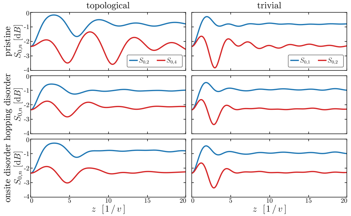
FIGURE A.2: Two-mode squeezing along the propagation axis ( \alpha = 0.3 , \xi = 0.9 ). Hopping and onsite disorder values used are d = 0.6v . The site at which the measurement is taken is indicated in the legend, which is valid for the entire column.
