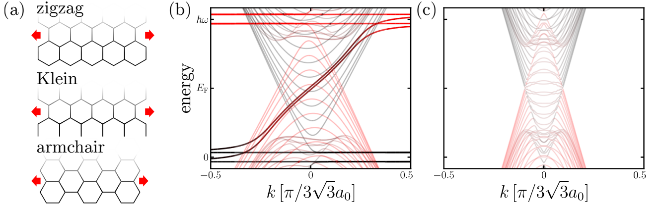
FIGURE E.1: (a) Scheme depicting the geometry of zigzag, Klein, and armchair edges, with red arrows marking the periodic direction. (b) Band structure of a Klein ribbon (of width 149a_0 ), showing two edge states with propagation direction contrary to those of a zigzag ribbon. (c) Band structure of an armchair ribbon (of width 100\sqrt{3}a_0 ). No edge states exist at the replica crossing. Color scale indicates the weight of the bands on n_{\text{ph}} = 0 (black) and n_{\text{ph}} = 1 (red), and transparency is relative to the localization.
