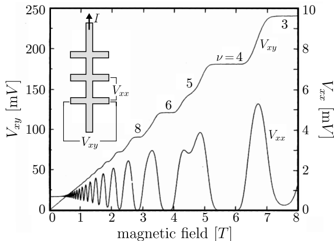
FIGURE 1.1: Hall voltage V_{xy} and longitudinal voltage V_{xx} as a function of the magnetic field in the IQHE. A scheme of the experimental setup is shown in the inset, with I the longitudinal current through the sample. Hall voltage takes quantized values V_{xy} = \frac{h}{\nu e^2 I} , exhibiting plateaus as a function of the magnetic field. Longitudinal voltage is in general zero, with peaks when the Fermi energy crosses a Landau level, and the Hall voltage changes value. Figure taken from [73].
