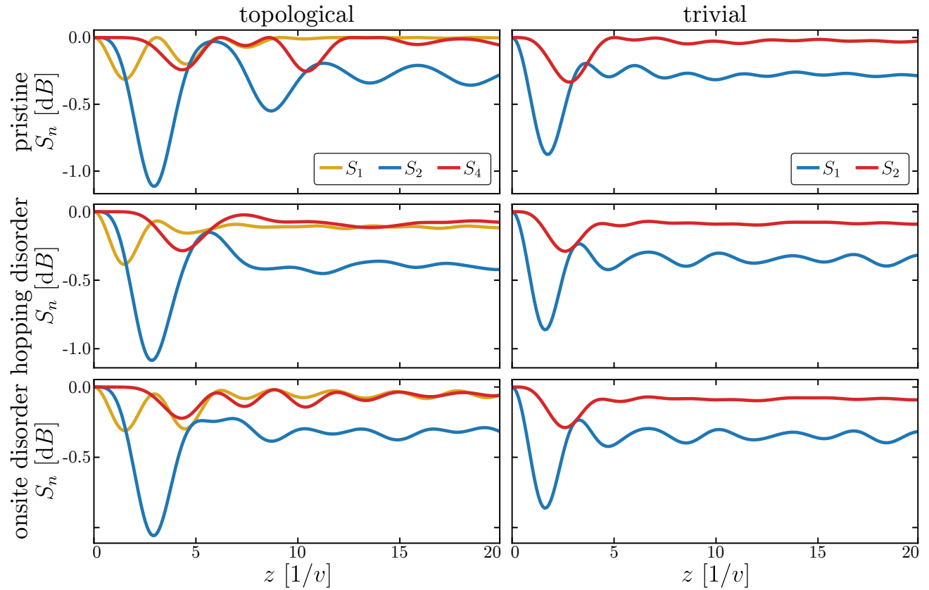
FIGURE A.1: One-mode squeezing along the propagation axis ( \alpha = 0.3 , \xi = 0.9 ). Hopping and onsite disorder values used are d = 0.6v . The site at which the measurement is taken is indicated in the legend, which is valid for the entire column.
