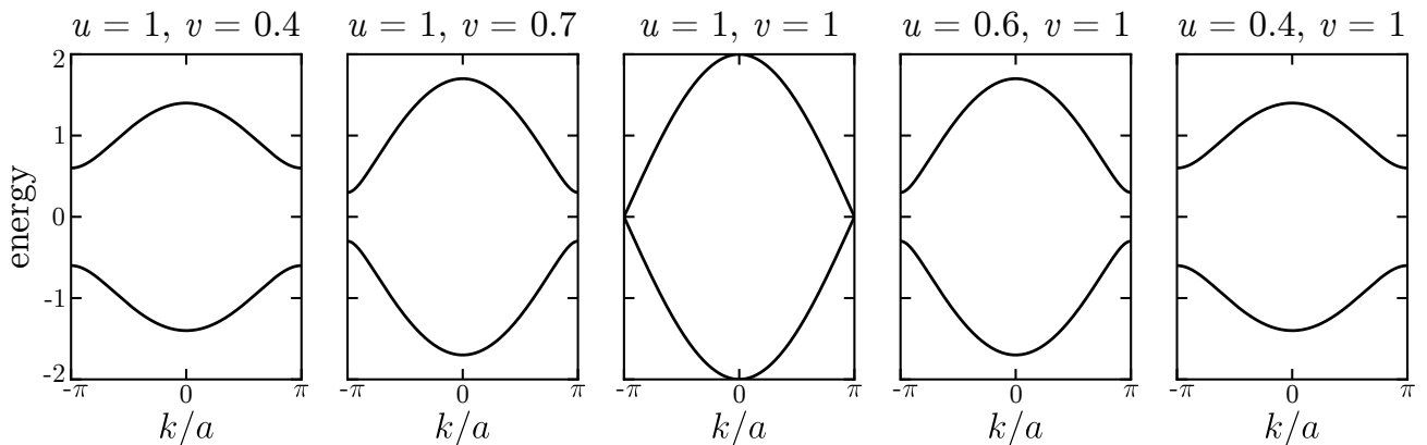
FIGURE 1.3: Energy bands of the SSH system. The hopping values u and v are indicated on top of each plot. The spectrum is invariant when interchanging u and v , and the gap only closes for |u| = |v| .
