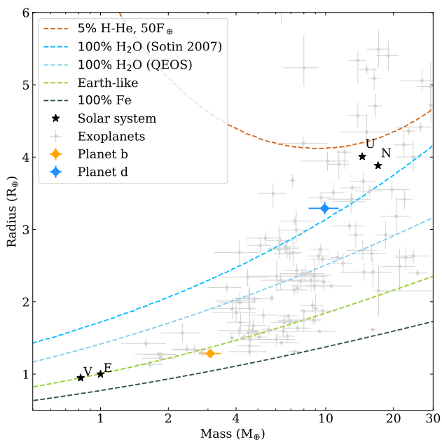
Figure 11. Mass-radius diagram of known exoplanets with mass determinations better than 4\sigma from the NASA exoplanet archive ( https://exoplanetarchive.ipac.caltech.edu , as of 22 September 2020) shown in grey. TOI-431 b (orange) and d (blue) are denoted as diamonds, and the Solar System planets Venus (V), Earth (E), Uranus (U), and Neptune (N) are marked as black stars. Also shown are the composition lines of iron (dark grey), Earth-like (green), and pure-water planets (pale blue and mid blue, using QEOS and EOS from Sotin et al. (2007) respectively), plus an additional line representing a planet with a 95 per cent water and a 5 per cent H-He envelope with F/F_\oplus = 50 , comparable to the case of the TOI-431 planets (brown).
