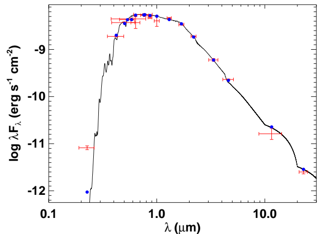
Figure 3. Spectral energy distribution (SED) of TOI-431. Red symbols represent the observed photometric measurements, where the horizontal bars represent the effective width of the passband. Blue symbols are the model fluxes from the best-fit Kurucz atmosphere model (black).
