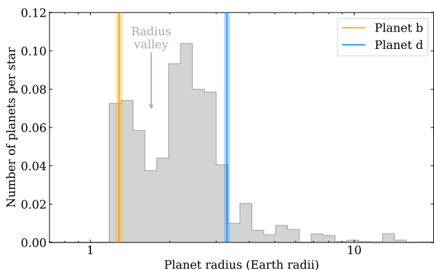
Figure 10. A histogram of planet radius for planets with orbital periods less than 100 days, as given in Fulton & Petigura (2018) . The radius valley can be seen at 1.7 R_{\oplus} : below the gap are rocky super-Earths, above the gap are gaseous sub-Neptunes. TOI-431 b (orange, with 1 \sigma confidence intervals shaded) is the former, while TOI-431 d (blue) is the latter.
