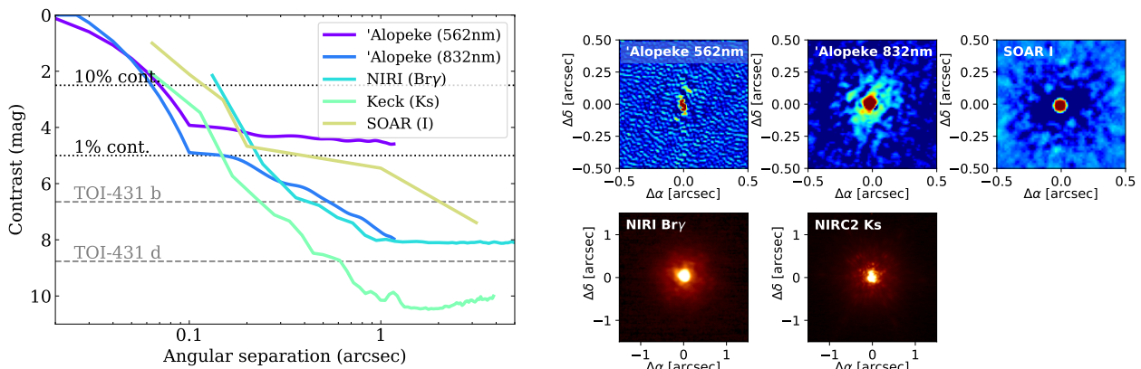
Figure 1. Left: 5\sigma contrast curves for all of the sources of high-resolution imaging described in Section 2.3. The 10 and 1 per cent contamination limits are given as the black dotted lines. The grey dashed lines labelled TOI-431 b and d represent the maximum contrast magnitude that a blended source could have in order to mimic the planetary transit depth if it were an eclipsing binary. Right: a compilation of reconstructed images from 'Alopeke and SOAR and AO images from NIRC2 and NIRC2, with the instrument and filter labelled. No additional companions are seen.
