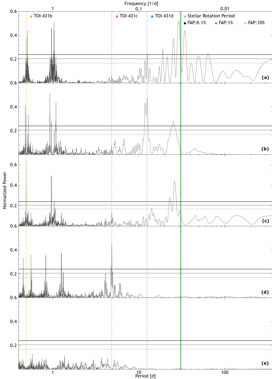
Figure 6. Periodograms for the HARPS data, where (going from top to bottom) the highest power peak has been sequentially removed until there is no power left. The best fit periods (see Table 3) of TOI-431 b (yellow), c (red), and d (blue), have been denoted by dotted lines, and the 1 standard deviation interval of the rotation period of the star has been shaded in green. The periodogram for the raw RV data is shown in panel (a); (b) has the stellar activity GP model removed; (c) has the best fit model for planet d removed also. Panel (d) has planet b removed, meaning that there should be no further power left. However, there is a peak evident at 4.85 days above the 0.1 per cent FAP that does not correlate with any stellar activity indicators, and it is not an alias of any other peaks. Taking this as an extra planet in the system (TOI-431 c) and removing the best fit model for this leaves a periodogram with no further signals, shown in panel (e).
