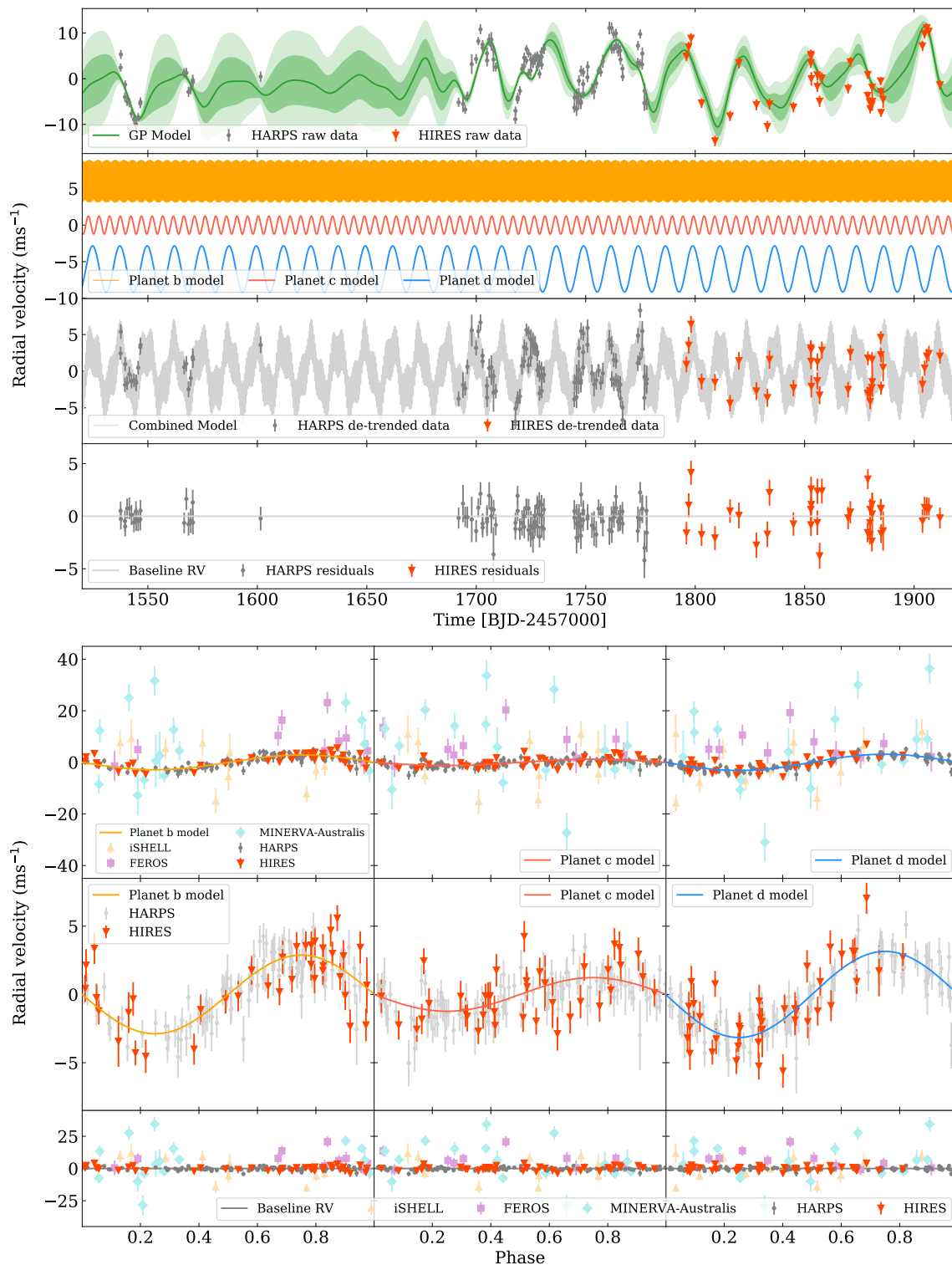
Figure 9. RV data plots, where the HARPS data is denoted as grey circles, HIRES as red upside down triangles, iSHELL as pale orange triangles, FEROS as pale pink squares, and MINERVA-Australis as pale turquoise diamonds. Top plot: the RV data, showing the GP and planet models that have been fit. Top: the best-fit GP used to detrend the stellar activity in the HARPS data is shown as the green line. The green shaded areas represent the 1 and 2 standard deviations of the GP fit. Upper middle: the separate models for each planet, b (orange, offset by +6 \text{ m s}^{-1} ), c (red), and d (blue, offset by -6 \text{ m s}^{-1} ). Lower middle: the total model, representing the addition of the models for planets b, c, and d, is plotted in black, and over plotted is the HARPS and HIRES data. Bottom: the residuals after the total model, GP and offsets have been subtracted from the RV data. Bottom plot: the phase folds for each planet model, b (left), c (middle), and d (right), with the RV data over plotted. The top row shows all of the RV data (where the GP has been subtracted from each data set), the middle just the HARPS and HIRES data, and the bottom the residuals when the planet models have been subtracted from the RVs.
