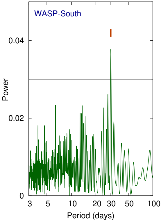
Figure 4. The periodogram of the WASP-South data for TOI-431 from 2012–2014. The orange tick is at 30.5 d, while the horizontal line is at the estimated 1 per cent false-alarm probability.
