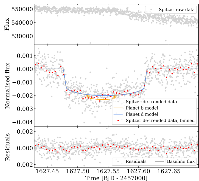
Figure 8. The Spitzer double-transit. Top: the raw Spitzer data, without any PLD applied. Middle: the Spitzer light curve detrended with PLD in grey and binned as red circles, with the best fit models of planet b (orange) and d (blue) overlaid. Bottom: the residuals when the best fit model has been subtracted from the detrended flux.
