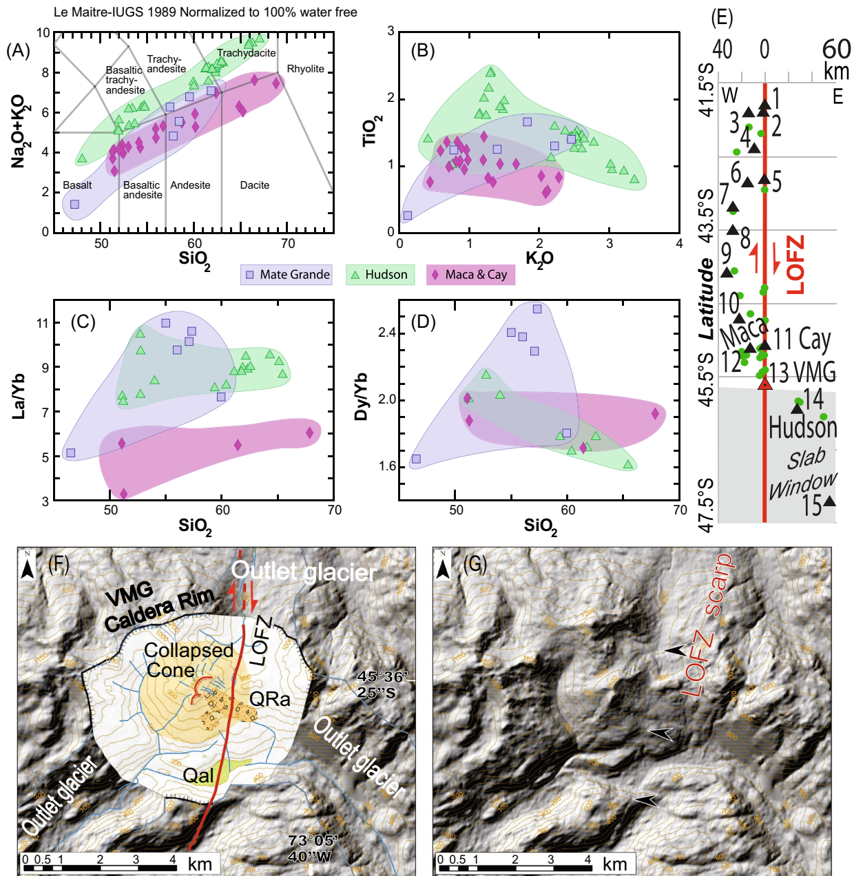
Figure 3. (A) Volcan Mate Grande (VMG; discovered during this study; 45^\circ 35' 28'' \text{S} , 73^\circ 07' 51'' \text{W} ) has Hi-K calcalkaline magmas and (B–D) distinct geochemical characteristics compared with Volcan Maca and Cay complexes (32, 33; VMCC: typical SVZ magmas) and Volcan Hudson (VH; atypical SVZ magmas). VMG has distinctive \text{La/Yb} (C) and \text{Dy/Yb} (D) values, i.e. a completely different signature between VMG magmas and VH magmas. (E) Distribution (perpendicular distance (km) and normalised along-strike of the LOFZ) of stratovolcanoes and monogenetic cones from 41.5^\circ to 47.5^\circ \text{S} based on our mapping. (F,G) DEMs and mapping from the VMG, showing the 5 km by 4 km caldera, the young partially collapsed cone, the rock avalanche deposits (QRa), Quaternary alluvium (Qal), and the location of the main trace of the LOFZ that cuts this cone and displaces the rock avalanche deposit (likely triggered by a LOFZ earthquake/rupture) northward (i.e. dextrally) by \sim 170 \pm 20 \text{ m} . Base hillshade was generated with Esri ArcMap v.10.3 software (under fair terms of use, https://www.esri.com/en-us/legal/copyright-trademarks ) 39 using a digital elevation model downloaded from ALOS PALSAR Global Radar Imagery 40 with 12.5 m resolution ( https://asf.alaska.edu/data-sets/sar-data-sets/alos-palsar/ ).
