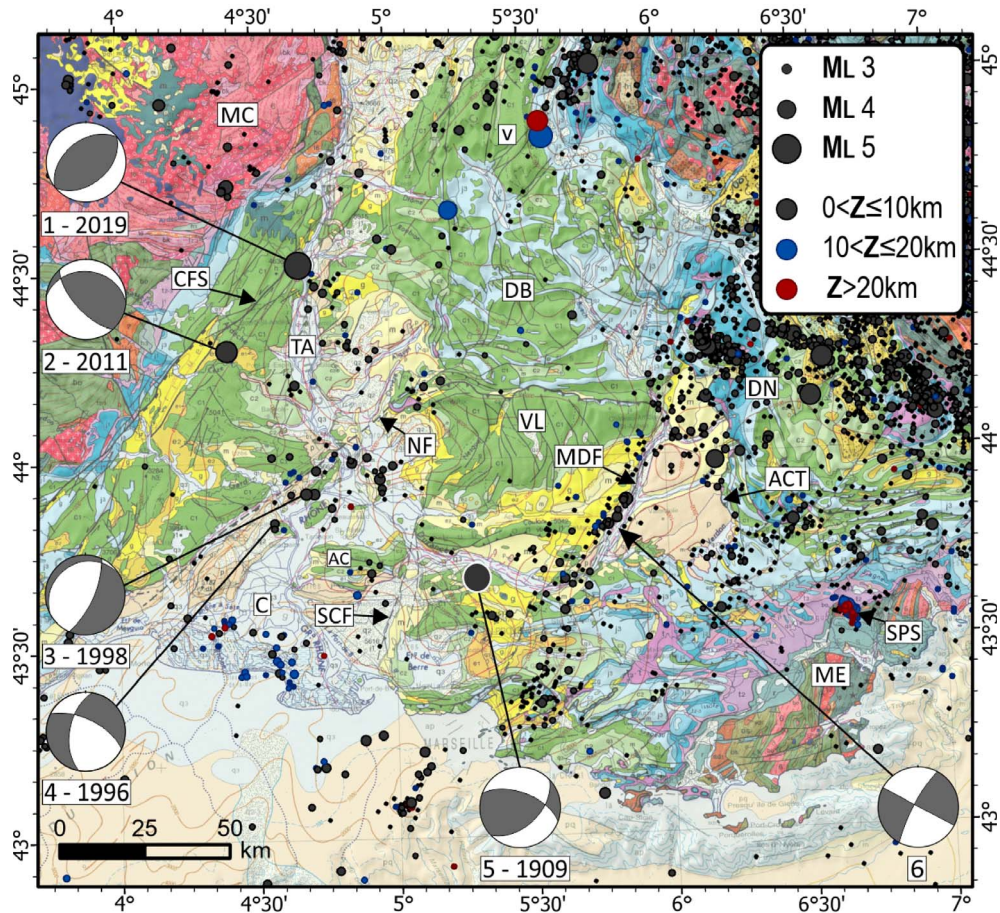
Figure 9. Seismicity overlaid on the geological map of the Southeast basin, from the CEA _1996–2019 catalog (all magnitudes, except for the 1909 Provence earthquake from Baroux et al. [2003]) and Chantraine et al. [2003]. Focal mechanisms: 1. Le Teil earthquake [2019/11/11, M_w 4.9; Ritz et al. , 2020]; 2. Largentière (2011/08/03, M_L 4.3; Delouis-Géoazur ); 3. [1998/02/09, M_L 3.1; Baroux et al. , 2001]; 4. [1996/03/25, M_L 3.1; Baroux et al. , 2001]; 5. Provence earthquake [1909/06/11, M_w 6.0; Baroux et al. , 2003]; 6. composite mechanism Durance fault [Cushing et al. , 2008].
