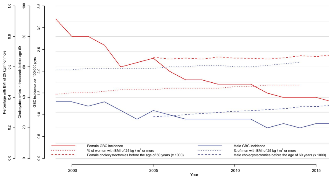
FIG. 4. Incidence of GBC, proportion of persons with BMI \geq 25 kg/m 2 , and number of cholecystectomies in Germany from 1999 to 2016 in women (red lines) and men (blue lines).
