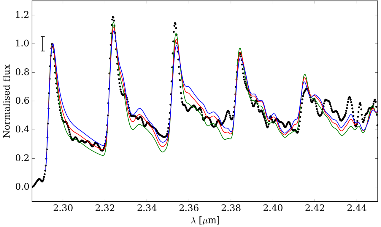
Fig. A.8. Same as Fig. A.4, but for models with fixed values of T = 2400 K, N_{\text{CO}} = 4 \times 10^{21} cm ^{-2} , and v_{\text{rot}} \sin i = 130 km s ^{-1} . Coloured solid lines represent models with different values of the intrinsic line width: \Delta v = 10 km s ^{-1} (solid green line), \Delta v = 15 km s ^{-1} (solid red line), and \Delta v = 20 km s ^{-1} (solid blue line). The data are smoothed at a resolution of R = 1000 . When the data are smoothed the first bandhead becomes smaller because the line peak has only a few points, which causes the second and third bandhead to exceed than the unsmoothed spectra when we normalise.
