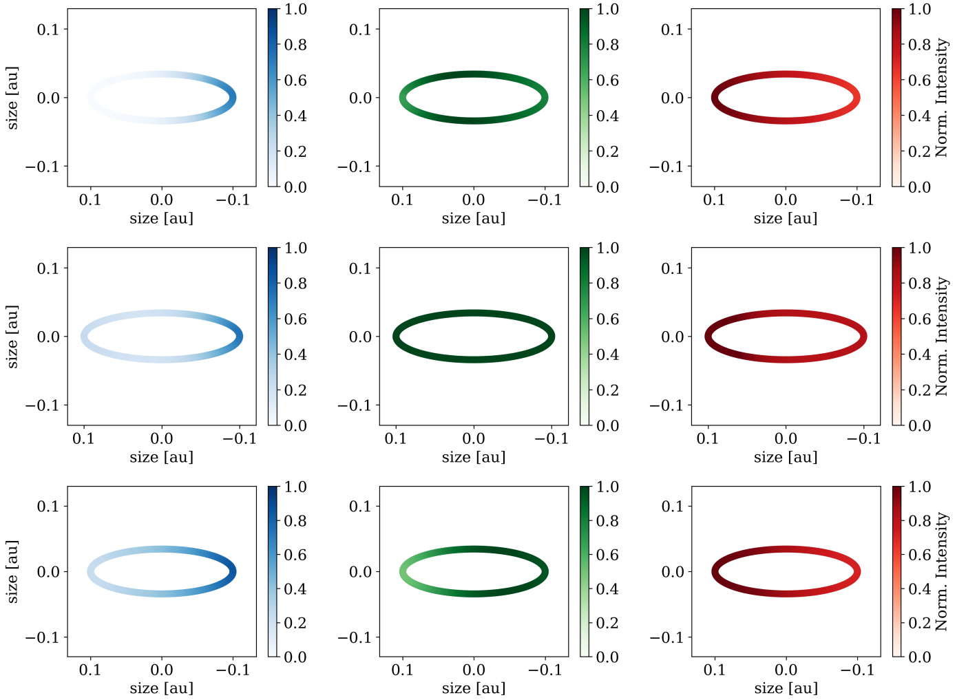
Fig. 9. Model-predicted intensity maps of the blue-shifted (average over spectral channels at 2.2925, 2.3213, and 2.3516 \mu\text{m} ), peak (average over spectral channels at 2.2945, 2.3237, and 2.3529 \mu\text{m} ), and red-shifted (average over spectral channels at 2.2954, 2.3246, and 2.3543 \mu\text{m} ) line components of the first ( top panel ), second ( middle panel ) and third ( bottom panel ) bandheads. Maps are normalised to the peak intensity and are displayed for an inclination of 70^\circ , and a radius of 0.1 au. The physical parameters of the model are the same as in Fig. 8.
