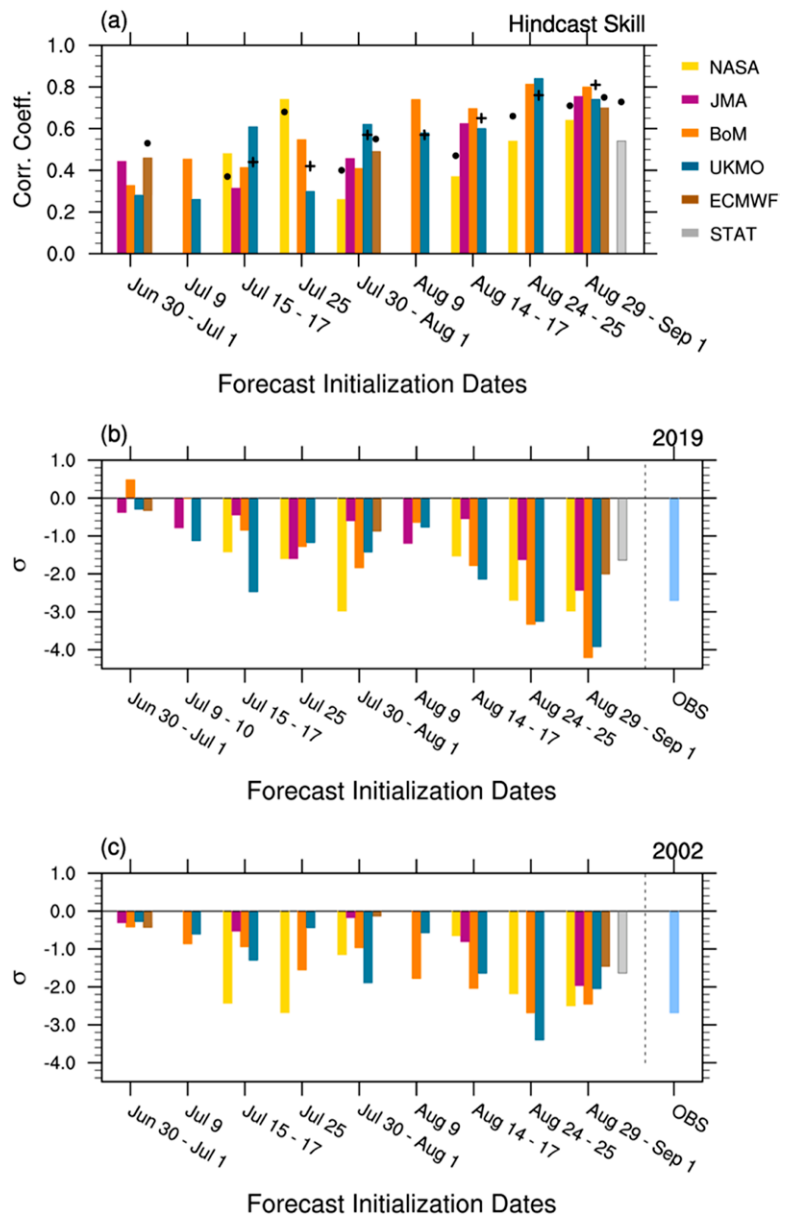
Fig. 9. (a) Hindcast skill to predict the SPVI (as defined with Fig. 2b; SON [U]' at 60^\circ\text{S} at 10 hPa) from the five different operational center S2S forecast systems: NASA GEOS-S2S-2 (yellow), JMA/MRI-CPS2 (purple), BoM ACCESS-S1 (orange), UKMO GloSea-5 (blue), and ECMWF-SEAS5 (brown). Skill of the statistical prediction discussed with Fig. 8 is displayed with gray bars. All colored bars, except for the blue bars (UKMO), represent the hindcast skill obtained over 1990–2012, for which the statistical model was rebuilt. The hindcast skill of the UKMO system was computed over 1993–2016. Black dots indicate the skill obtained over longer hindcast periods (see Table 1). The crosses overlaid with the blue bars indicate the skill with an increased ensemble size by using up to 17-day lags (compared to seven-member burst ensemble used for the skill shown with the blue bars). (b),(c) Dynamical and statistical forecasts of standardized SPVI for 2019 and 2002, respectively. The observed anomalies are displayed with light blue bars. All the forecast anomalies were computed with each system's climatological mean and standard deviation from its hindcast periods. The abscissa labels show the forecast initialization dates. Displayed dynamical forecasts are the ensemble mean forecasts (except for NASA forecasts), and details of the forecast systems and ensemble sizes are provided in Table 1.
