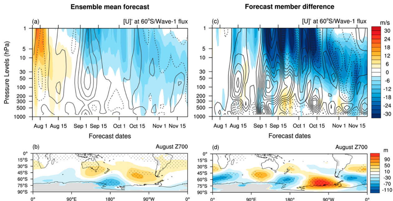
Fig. 10. The 11-member ensemble-mean forecasts of (a) daily [U]' at 60^\circ\text{S} (color shading) overlaid with standardized upward wave-1 activity flux ( F'_{(p)} ) (contours) and (b) August-mean Z700 anomalies (color shading) from the BoM system. Forecasts were initialized on 25 Jul 2019. In (a) the solid (dashed) thick contour indicates the poleward (equatorward) heat flux and so upward (downward) wave propagation. Normalization of the wave activity flux by its standard deviation was done at each vertical level. Stippling in (b) indicates anomalies at the \pm 5\% tails of the climatological distribution of BoM hindcasts. (c),(d) As in (a) and (b), respectively, but for the mean differences between the three forecast members of the weakest spring polar vortex and those of the strongest spring polar vortex. The color shading interval is 3 \text{ m s}^{-1} , and the contour interval is 1\sigma starting from -11.5\sigma in (a) and (c). The color shading interval is 20 m in (b) and (d). Stippling in (d) indicates statistical significance on the difference of the two means at the 10% level, assessed by a two-tailed Student's t test with the sample size of three in each group.
