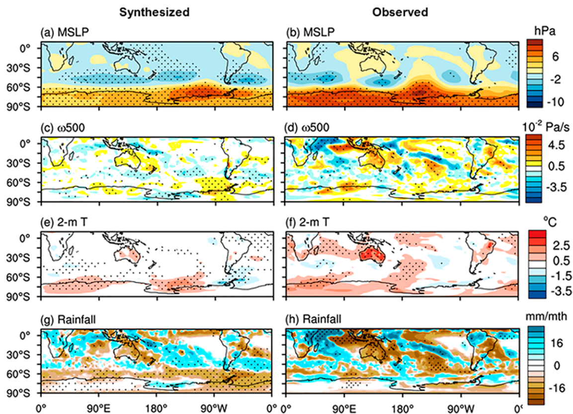
Fig. 6. Syntheses of 2019 OND-mean (a) mean sea level pressure (MSLP), (c) vertical velocity ( \omega ) at 500 hPa, (e) 2-m air temperature, and (g) rainfall anomalies derived from the regression onto the SPVI as described in Fig. 3. The color shading interval is 2 hPa in (a), 0.01 Pa s -1 in (c), and 1°C in (e). The color shading interval in (g) increases by twofold for each level from –2 and 2 mm month -1 . (b),(d),(f),(h) As in (a), (c), (e), and (g), but the observed anomalies of 2019. Stippling indicates the statistical significance as described in Fig. 3, except in (h), where stippling shows where the rainfall anomalies are found in the top- and bottom-decile categories.
