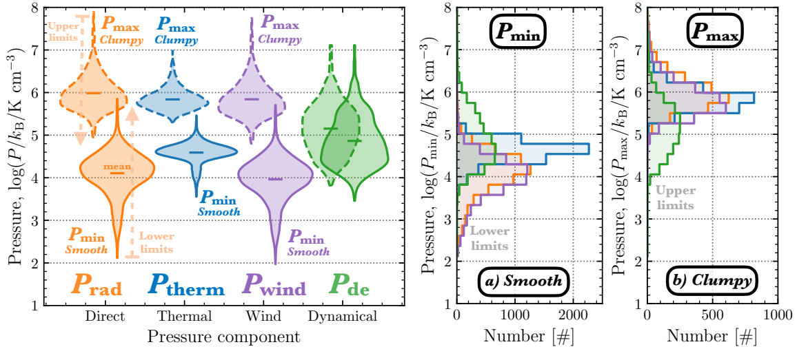
Figure 9. Distribution of the various pressure components determined across the H II region sample for all galaxies for assumptions of a a) smooth and b) clumpy unresolved density distribution (see Figure 2). We show the internal pressure components of the direct radiation pressure ( P_{\text{rad}} ) in orange, thermal pressure from the ionised gas ( P_{\text{therm}} ) in blue, and ram pressure from the wind ( P_{\text{wind}} ) in purple. We show the distribution of the external confining pressure or dynamical pressure ( P_{\text{de}} ) in green. Left panel: The KDE distributions are represented as violin plots, where the mean value of each distribution is highlighted by a horizontal bar and the width of each distribution corresponds to the logarithmic scale histogram distribution. The distributions for both the maximum pressure limit ( P_{\text{max}} ) calculated for the smallest volume, and minimum pressure limit ( P_{\text{min}} ) calculated for the largest volume are shown with dashed and solid outlines, respectively. The dashed, faded arrows highlight that P_{\text{max}} and P_{\text{min}} represent upper and lower limits on the internal pressure. Right panels: We show the histogram distributions for P_{\text{min}} and P_{\text{max}} separately.
