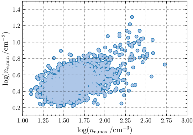
Figure A1. Comparison the electron densities assuming a smooth ( n_{e,\min} ) and clumpy ( n_{e,\max} ) unresolved density distribution (see Figure 2). We plot H II regions for which we can derive both r_{\min} and n_{e,\min} (2238 regions in total; see section 3.4).
