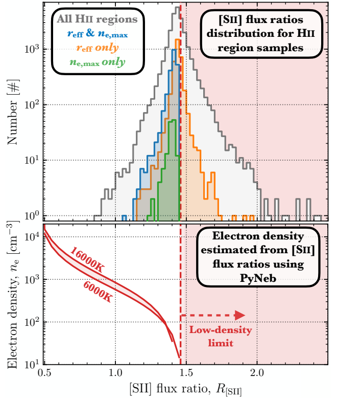
Figure 4. Upper panel: Histogram of the R_{[\text{SII}]} = F_{[\text{SII}]\lambda 6716}/F_{[\text{SII}]\lambda 6731} line ratio across the H II region sample. We show the distribution of R_{[\text{SII}]} for the full sample of H II regions as a grey histogram. The vertical dashed red line and shaded region shows the low-density limit (also shown in the lower panel). The blue and green histograms show the distributions of H II regions that are statistically distinguishable from the low-density limit (see Figure 6), and have resolved and unresolved sizes (see Section 3.1). The orange histogram shows the H II regions that are indistinguishable from the low-density limit, yet are resolved (see Figure 6). Lower panel: The dashed curve shows the conversion between R_{[\text{SII}]} and electron density ( n_e , see right y-axis) as determined from PyNEB assuming two electron temperatures that span the observed range of approximately 6000 K to 16,000 K.
