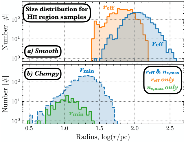
Figure 3. Histograms of the size distribution for the H II region sample for assumptions of a a) smooth and b) clumpy unresolved density distribution (see Figure 2). Upper panel: We show r_{\text{eff}} for the resolved ( r_{\text{eff}} \geq \text{FWHM}_{\text{PSF}} ; see Section 3.1) sources as both blue (solid outline) and orange histograms. The blue and orange histograms differentiate the samples with and without n_{e,\text{max}} electron density measurements, respectively (see Section 3.2). Lower panel: Where possible, we also determine a size ( r_{\text{min}} ) using the n_{e,\text{max}} determined from R_{[\text{SII}]} and the H \alpha flux (see Section 3.4). These r_{\text{min}} distributions are shown in green and blue (dashed line). Note that the H II regions that are both resolved and are below the low-density limit have both r_{\text{min}} and r_{\text{eff}} estimates, and, hence, the blue histograms have the same sample size.
