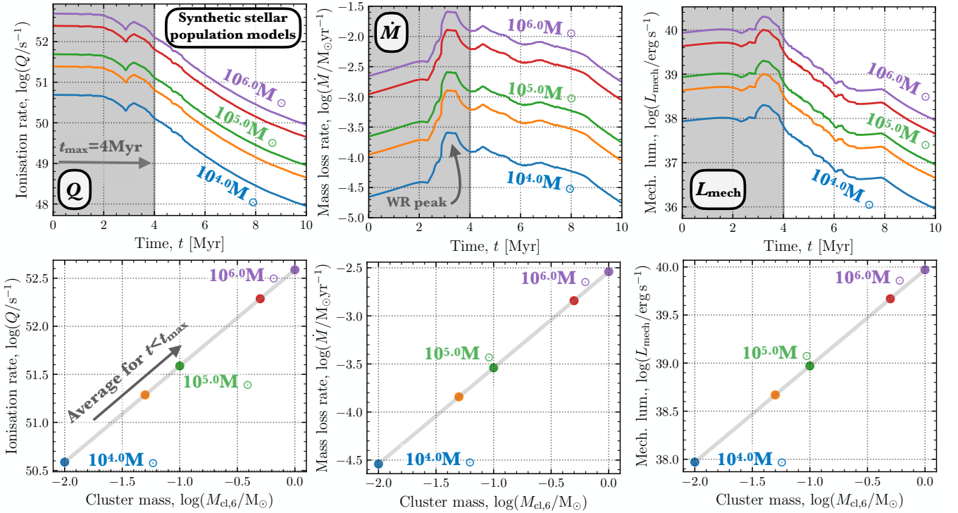
Figure 8. Upper panels (left to right): Early time evolution of the ionisation rate ( Q ), mass loss rate ( \dot{M} ), and mechanical luminosity ( L_{\text{mech}} ) from the STARBUST99 model (Leitherer et al. 1999) for cluster with masses of M_{\text{cl}} = 10^4 to 10^6 M_\odot . The shaded region represents t < t_{\max} , where t_{\max} is the time for L_{\text{H}\alpha} to drop by half an order of magnitude from the zero-age main sequence (see Section 3.5.1). We label the peak in the mass loss rate seen at \sim 3.5 Myr that corresponds to the time at which winds are the most effective (Leitherer et al. 1999; Rahner et al. 2017, 2019), as the most massive O stars are in their Wolf–Rayet phase but have not yet exploded as supernovae. Lower panels (left to right): The average Q , \dot{M} and L_{\text{mech}} between t = 0 Myr and t_{\max} = 4 Myr plotted as a function of the cluster mass ( M_{\text{cl},6} = M_{\text{cl}}/10^6 M_\odot ). We use the measured Q for each H II region to infer M_{\text{cl}} . We then use this M_{\text{cl}} to estimate L_{\text{mech}} and \dot{M} , which are used in the calculation of the wind ram pressure ( P_{\text{wind}} ; see Section 4.1.2).
