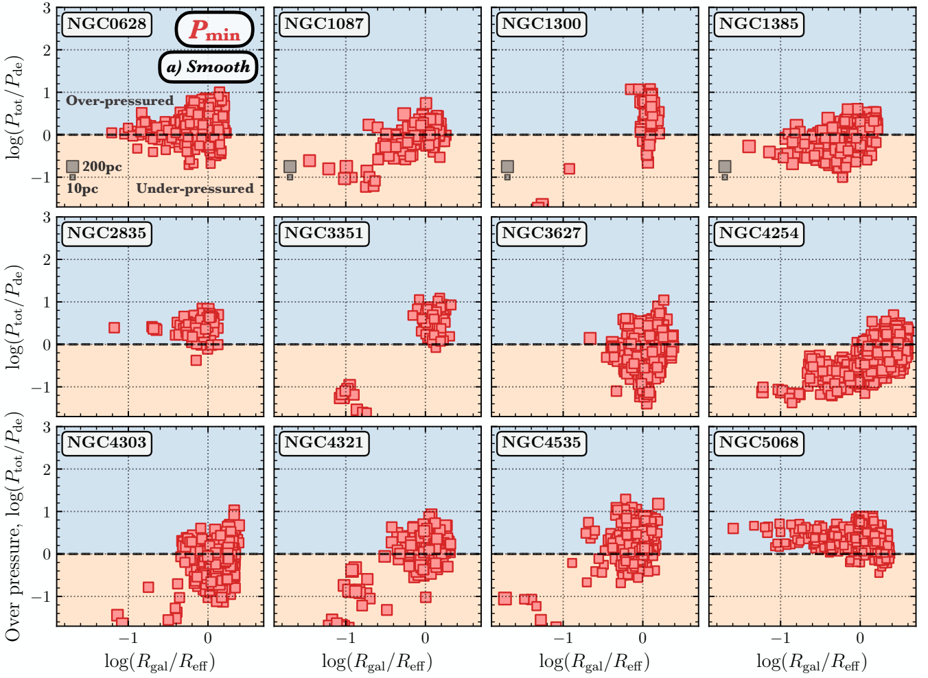
Figure 14. Over-pressure, P_{\text{tot}}/P_{\text{de}} = (P_{\text{therm}} + P_{\text{wind}} + P_{\text{rad}})/P_{\text{de}} , of each H II region as a function of the galactocentric radius for each galaxy for assumptions of a) smooth and b) clumpy unresolved density distribution (see Figure 2). We plot the galactocentric radius normalised to the R_{\text{eff}} radius (see Table 1). The size of each point has been scaled to the radius of the H II region, and corresponds to the scale shown in the lower left of each panel. The horizontal dashed black line shows where the external pressure is equal to the internal pressure. Above the dashed line the H II regions would be over-pressured (blue shaded), and below the H II regions are under-pressured (orange shaded).
