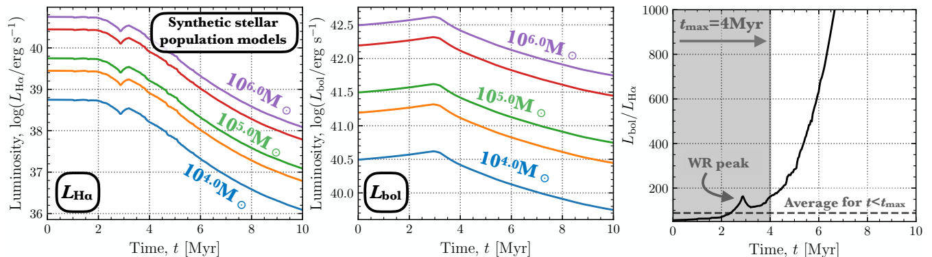
Figure 7. Early time evolution of the luminosity from the STARBURST99 model (Leitherer et al. 1999). Left and centre panels: We show the H \alpha luminosity ( L_{\text{H}\alpha} ) and the bolometric luminosity ( L_{\text{bol}} ) for cluster with masses of M_{\star} = 10^4 to 10^6 M_{\odot} , in steps of 0.5 dex. Right panel: We show the ratio of L_{\text{bol}}/L_{\text{H}\alpha} , which is the same for all cluster masses. We label the average L_{\text{bol}}/L_{\text{H}\alpha} \sim 88 between t = 0 Myr and t_{\text{max}} = 4 Myr, where t_{\text{max}} is the time for L_{\text{H}\alpha} to drop by half an order of magnitude from the zero-age main sequence (see Section 3.5.1). We also label the peak in the mass loss rate seen at \sim 3.5 Myr that corresponds to the time at which winds are the most effective (Leitherer et al. 1999; Rahner et al. 2017, 2019), as the most massive O stars are in their Wolf–Rayet phase but have not yet exploded as supernovae. The estimate of L_{\text{bol}} from L_{\text{H}\alpha} for each H II region is used in the calculation of the direct radiation pressure ( P_{\text{rad}} ; see Section 4.1.1).
