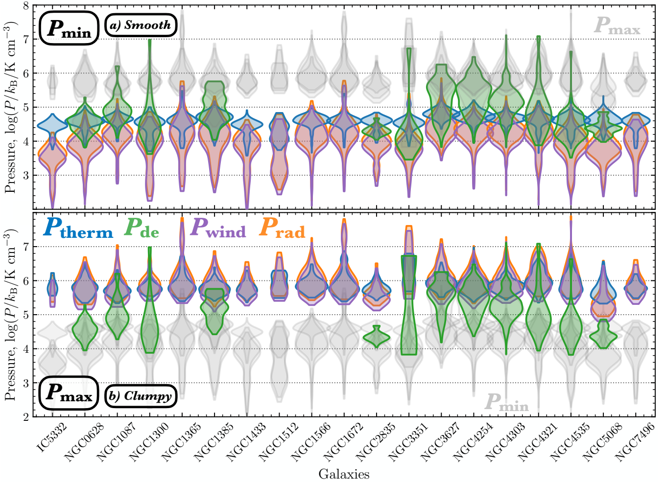
Figure 10. Distribution of the various pressure components determined across the H II region sample within individual galaxies for assumptions of a a) smooth and b) clumpy unresolved density distribution (see Figure 2). We show the internal pressure components of the direct radiation pressure in orange ( P_{\text{rad}} ), thermal pressure from the ionised gas in blue ( P_{\text{therm}} ), and ram pressure from the wind in purple ( P_{\text{wind}} ). Note that several galaxies were not included in the sample from Sun et al. (2020) due to no available H I observations or due to the lack of significant CO emission (e.g. IC 5332), and hence have no P_{\text{de}} measurement. We show the distribution of the external confining pressure, or dynamical pressure ( P_{\text{de}} ), in green. The KDE distributions are represented by violin plots, where the width of each distribution corresponds to the logarithmic scale histogram distribution. Upper panel: The distributions for the maximum pressure limit ( P_{\text{max}} ) are shown in colour, and minimum pressure limit ( P_{\text{min}} ) in faded grey. Lower panel: The distributions for the P_{\text{min}} are shown in colour, and P_{\text{max}} in faded grey.
