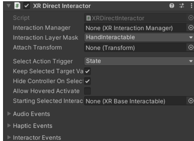
Figura 4.5: Componente XR Direct Interactor
