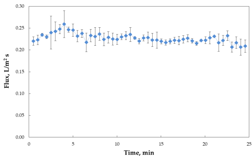
Figure 9. Variation of permeate flux with time, obtained in the UF stage for gypsum formed after neutralization at pH 10.5.
